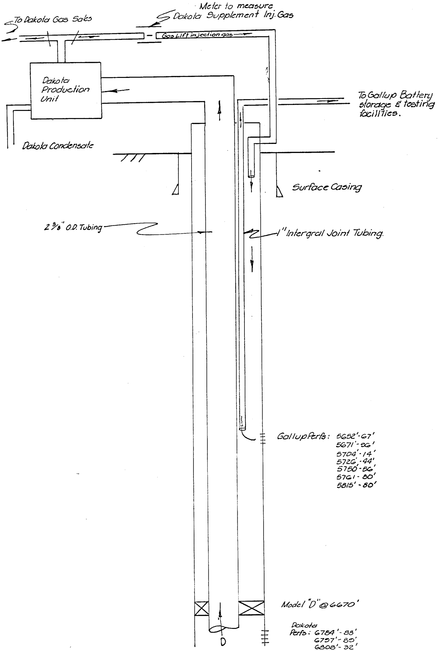
SCHMATIC DIAGRAM NO. 2 PROPOSED DUAL COMPLETION NE. HAYNES NO. 8 UNIT P, Section 15, T24N, R5W Rio Arriba Co, New Mex.
