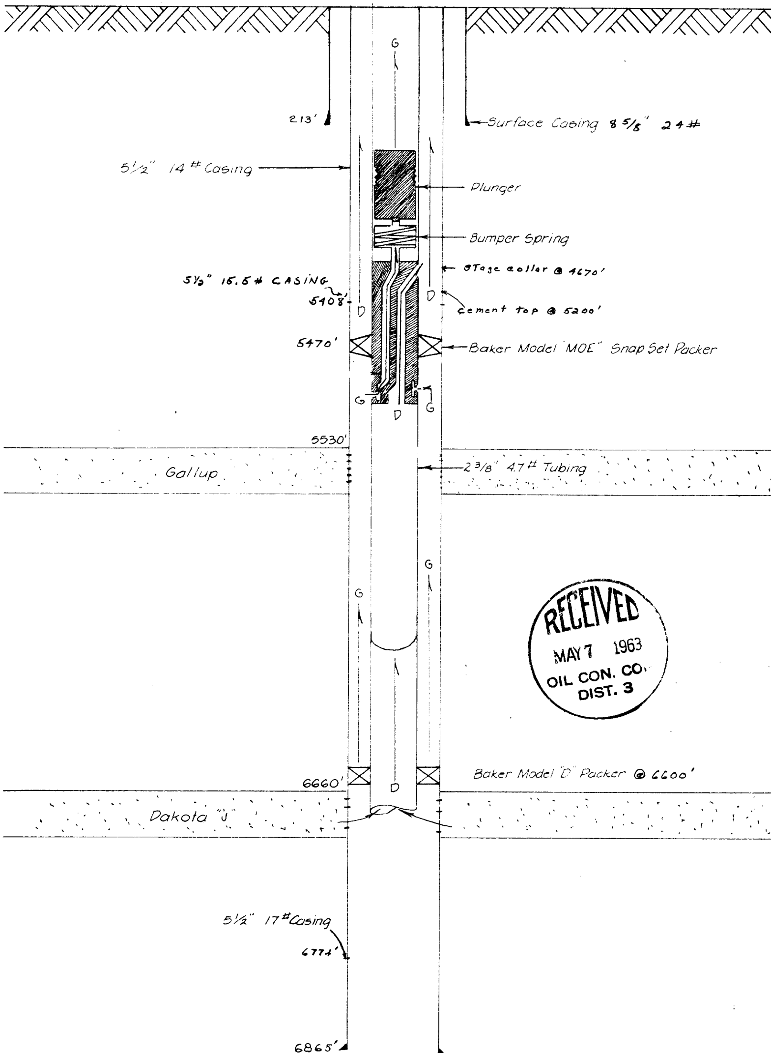
SCHEMATIC DIAGRAM of DUAL COMPLETION of NE HAYNES No. 2 CONTINENTAL OIL CO. Dakota & Gallup Formations.
