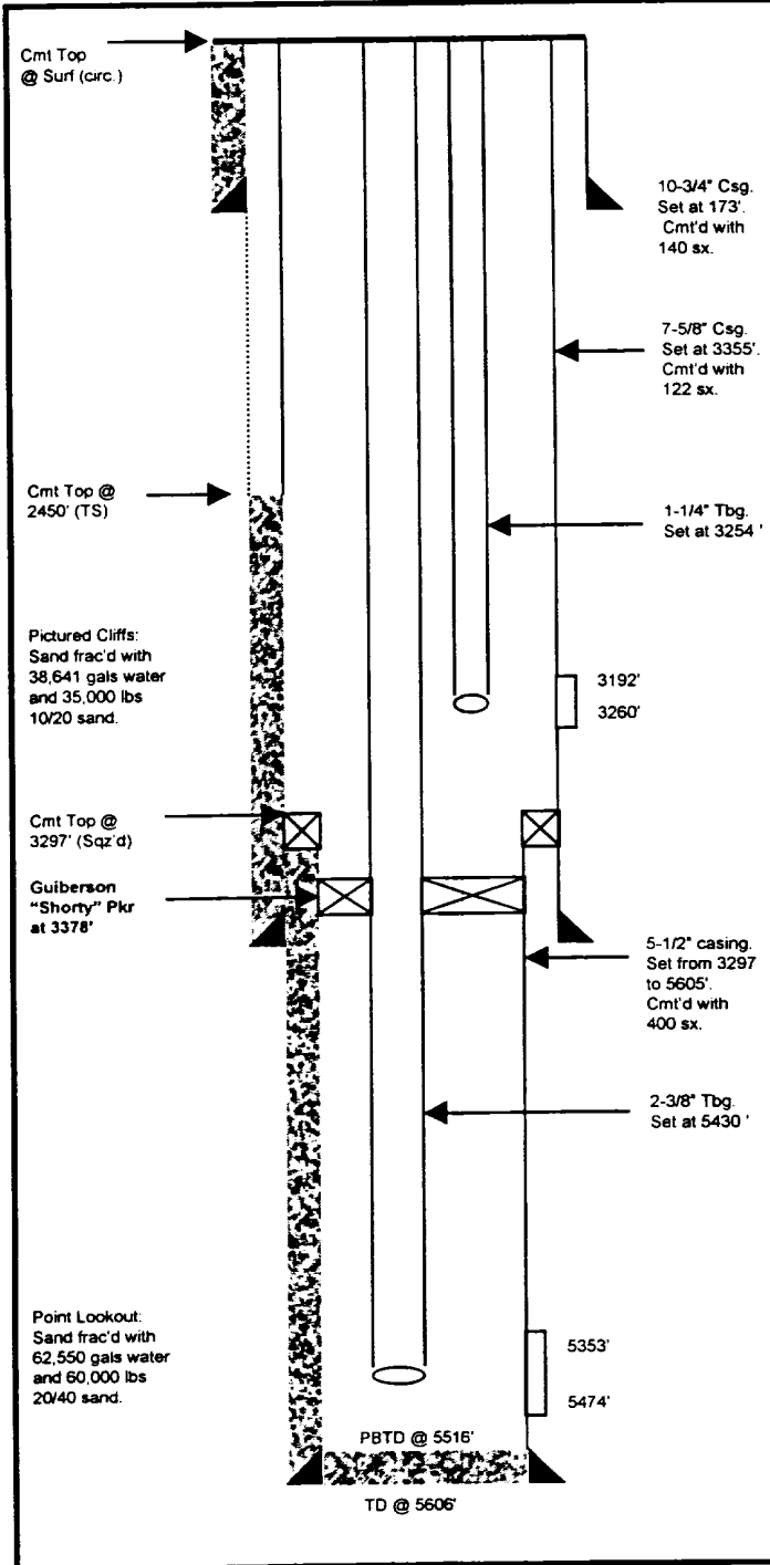
Current Schematic
