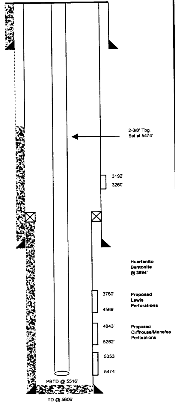
Proposed Schematic
