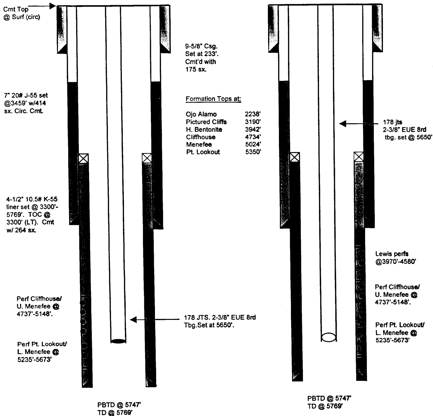
Current Schematic
