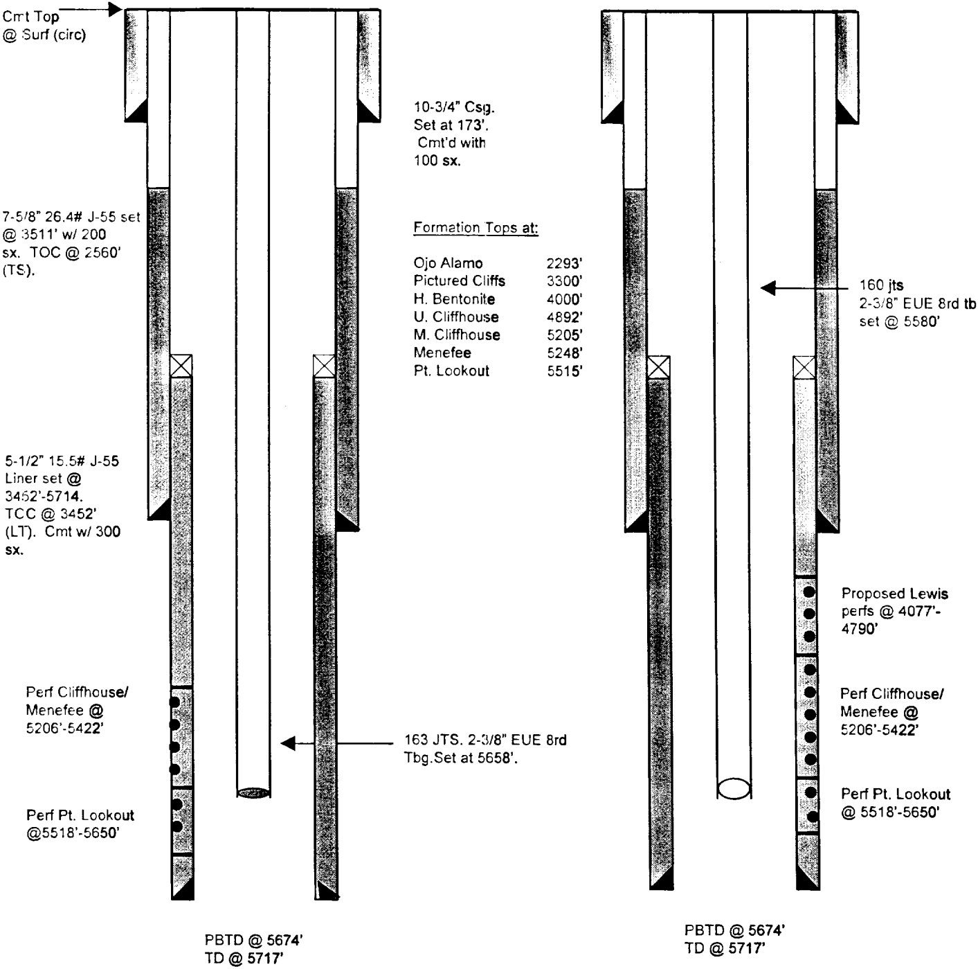
Current Schematic
