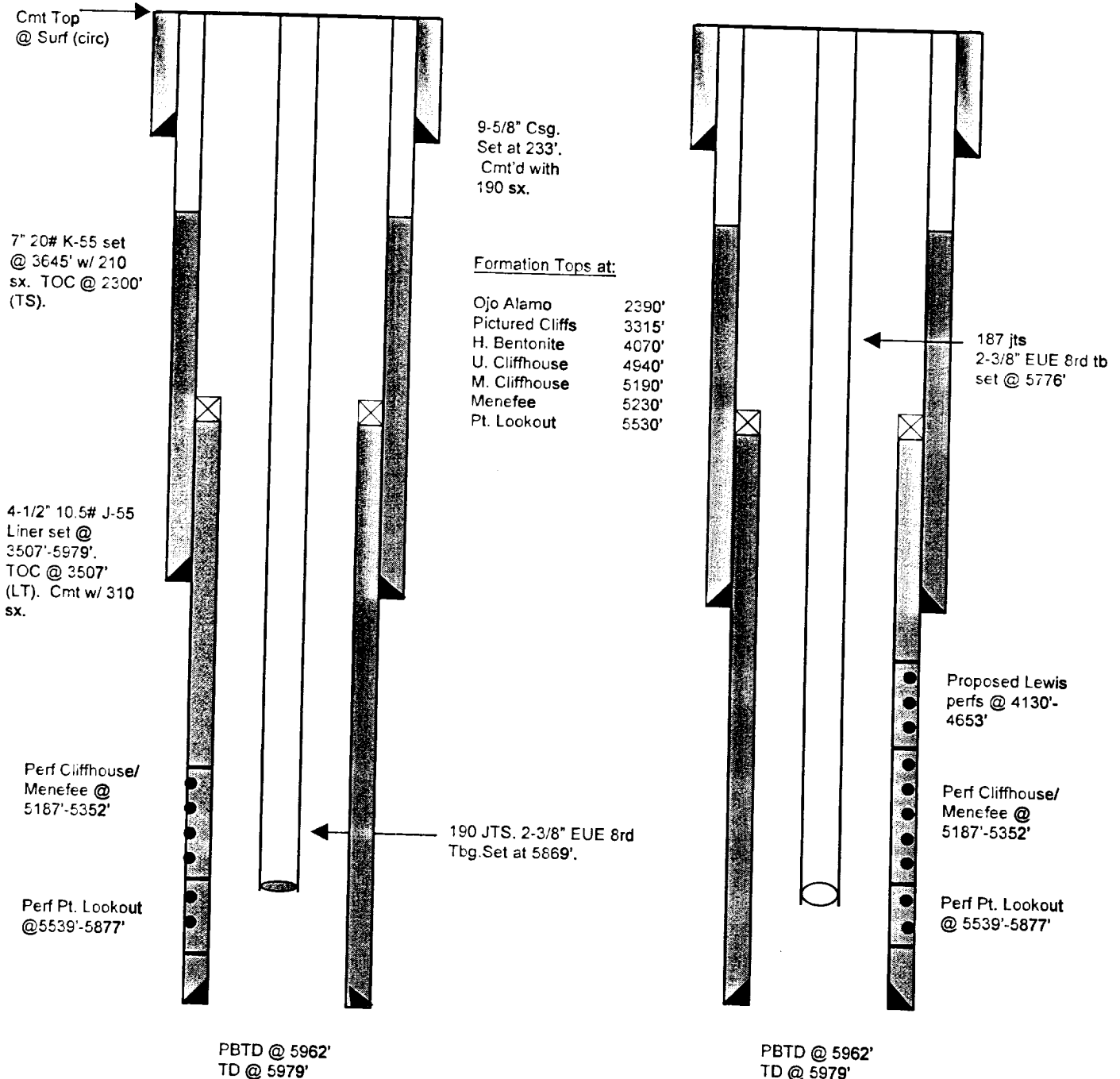
Proposed Schematic
