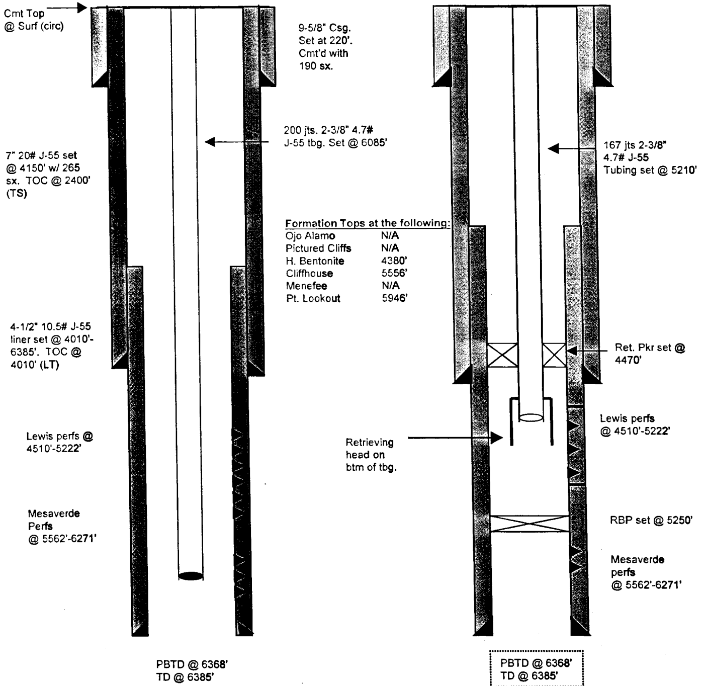
After Well Test Schematic
