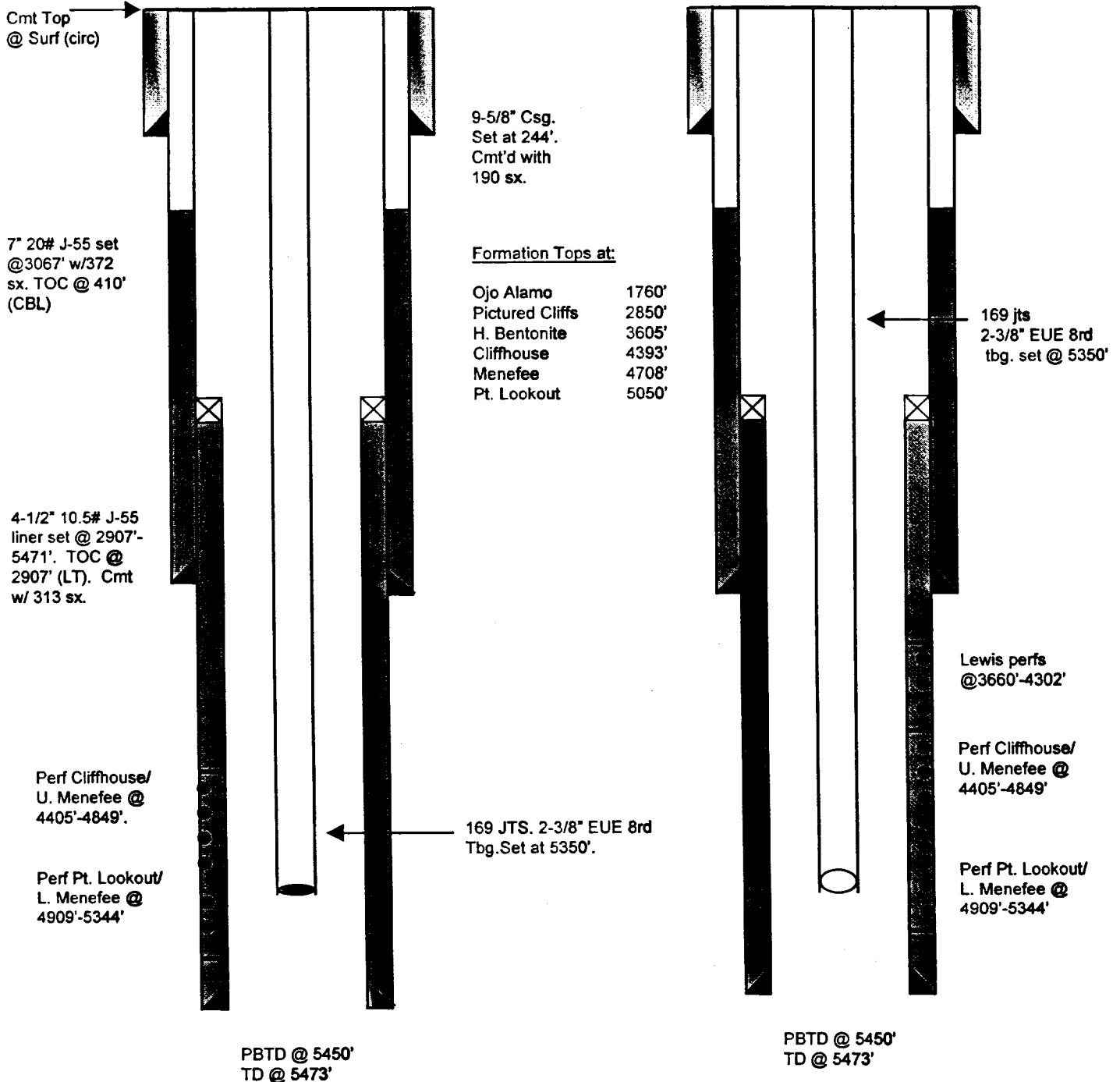
Current Schematic
