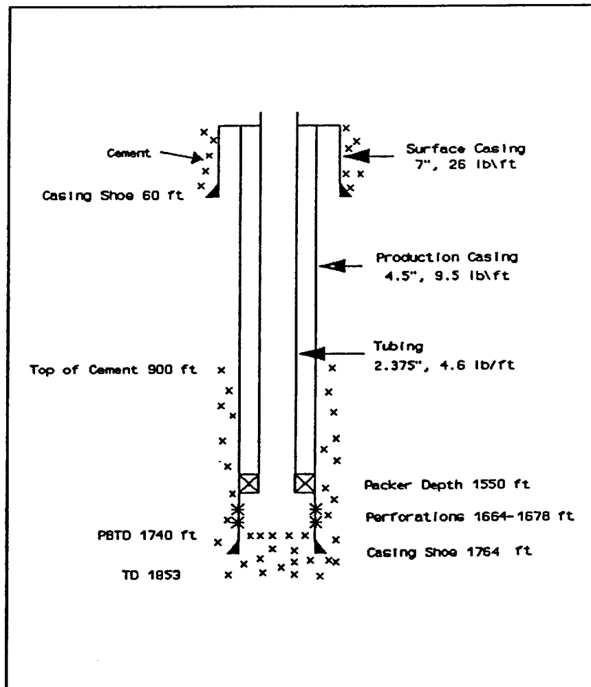
Figure 1 Construction schematic for the well Navajo #5. All depths are in feet below the surface.
