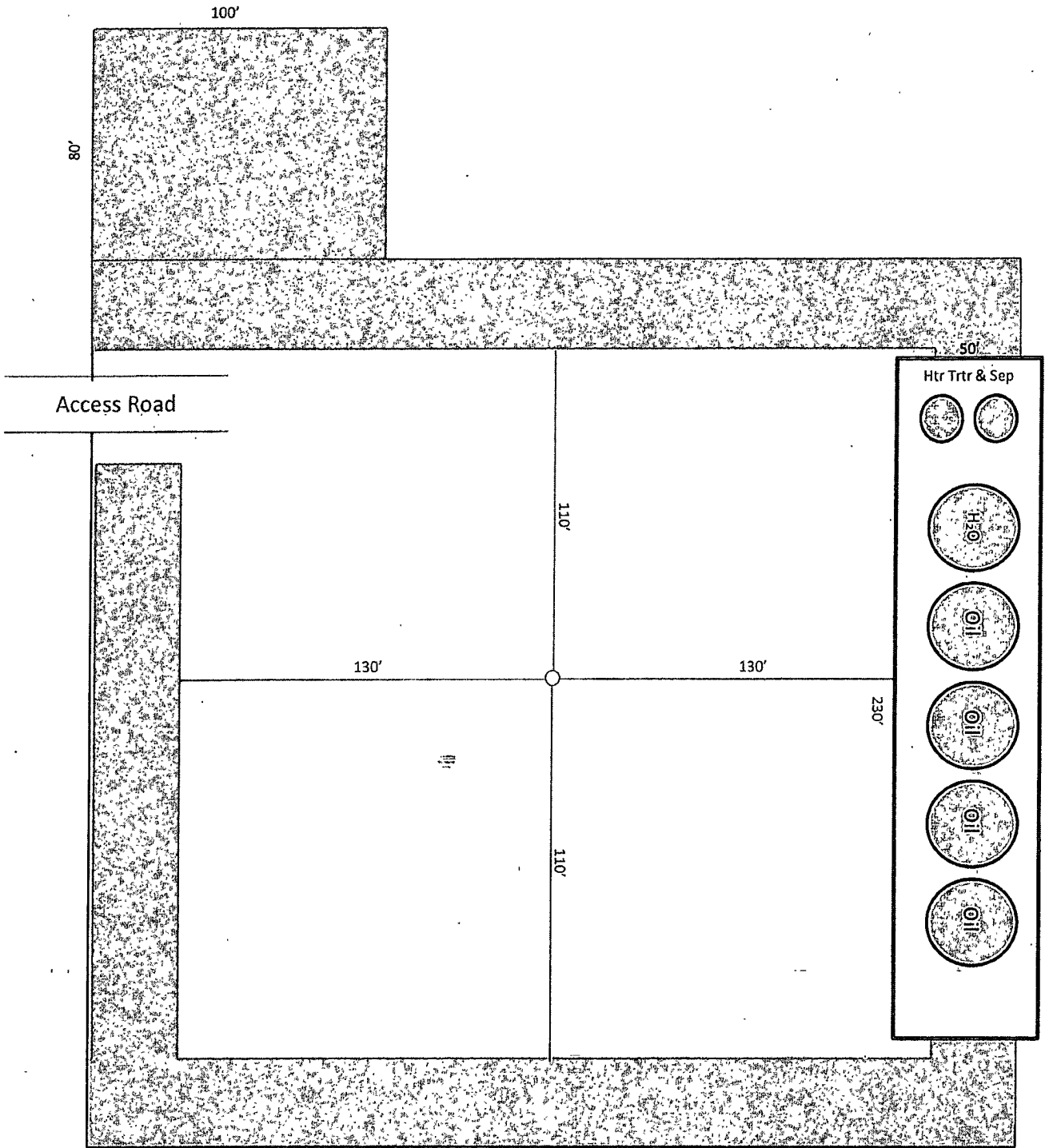
Exhibit D-1 Production Facilities Layout Diagram Cuervo Federal No. 20H Cimarex Energy Co. of Colorado 14-23S-32E SHL 330 FNL & 375 FEL BHL 330 FSL & 375 FEL Lea County, NM
