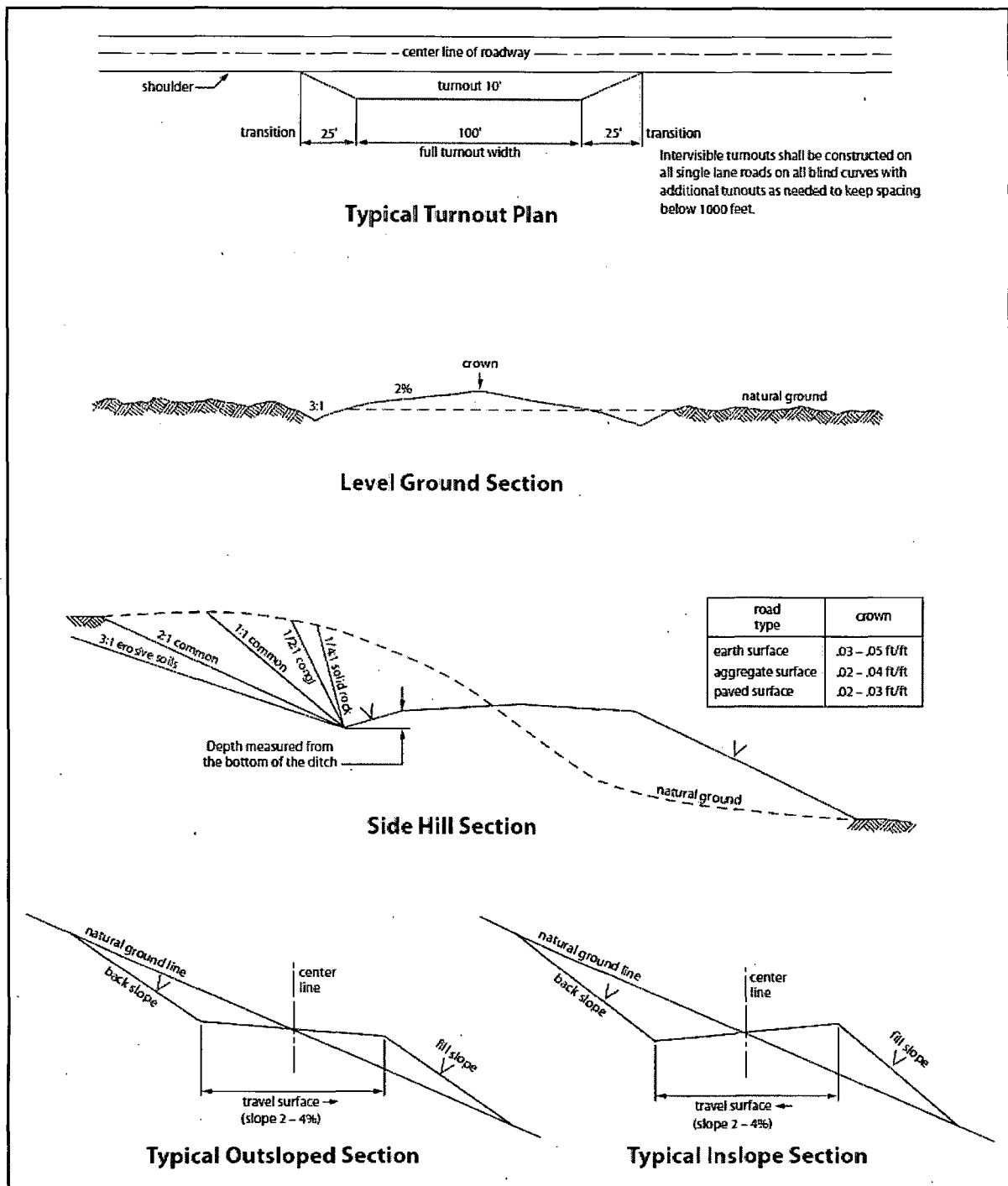
Figure 1. Cross-sections and plans for typical road sections representative of BLM resource or FS local and higher-class roads. DRILLING
