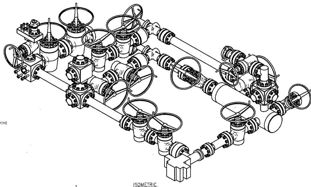
ISOMETRIC
