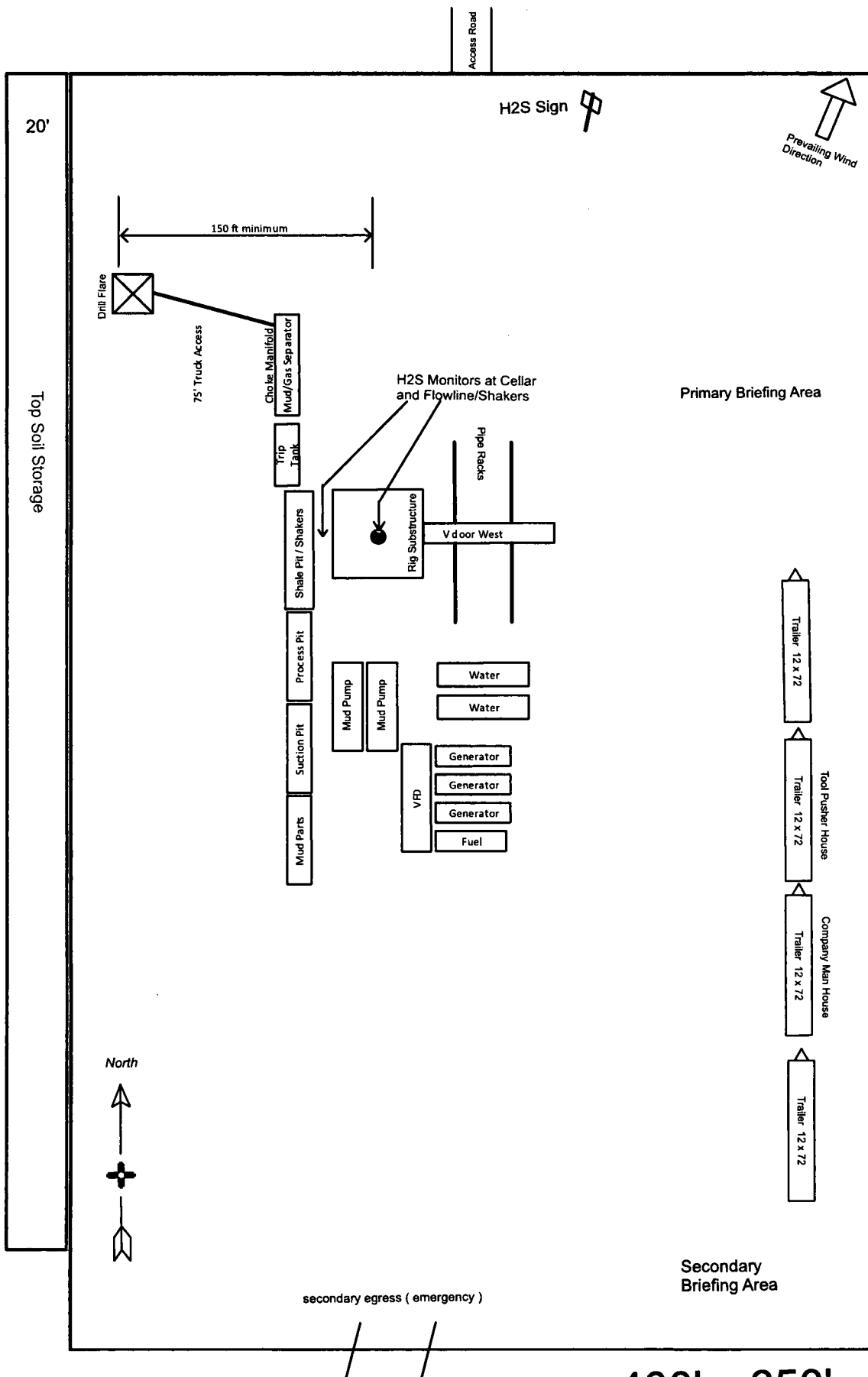
General Drill Site Layout
