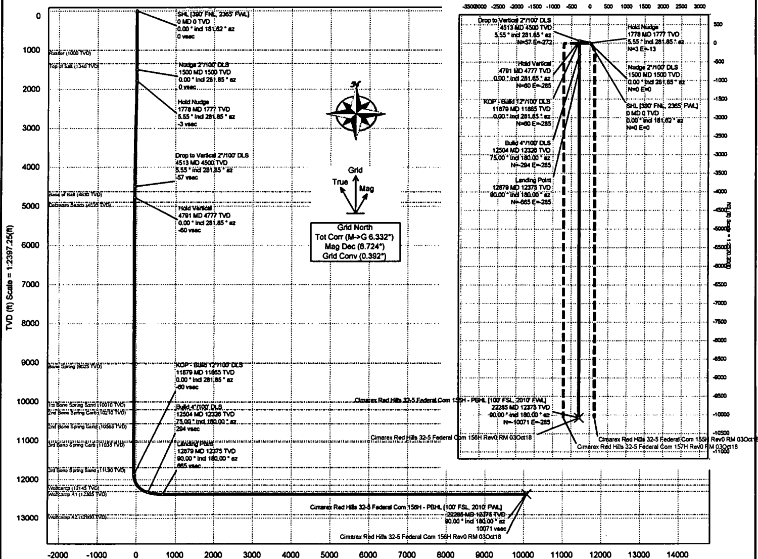
Vertical Section (ft) Azim = 180.00° Scale = 1:2397.25(1) Origin = 0N-S, 0E-W
