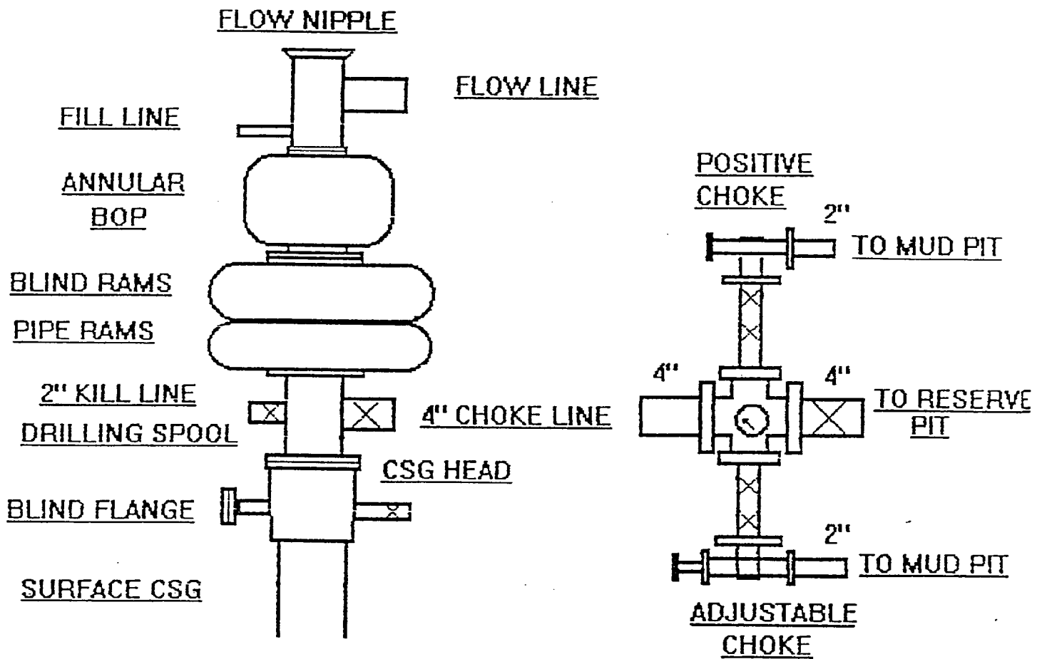
BOP AND CHOKE DIAGRAM
