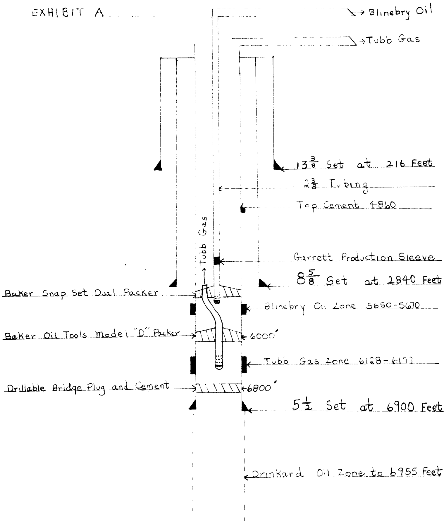
Diagram of Proposed Blinebry Oil - Tubb Gas Dual
