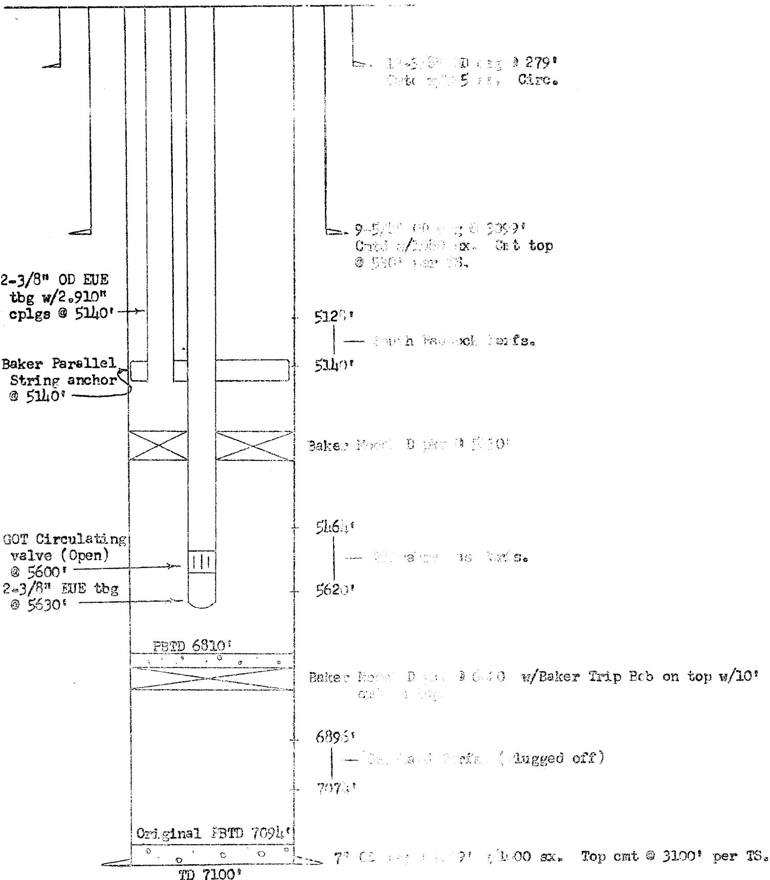
DIAGRAMATIC SKETCH OF PROPOSED DUAL COMPLETION GULF OIL CORPORATION - BARNBOROUGH ESTATE NO. 3-I Blinebry Gas & South Padonch Oil Pools Sec. 31, T-28-N, R-10-E
