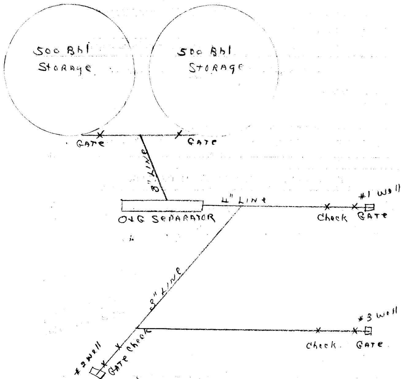
Diagram of hook-up:
