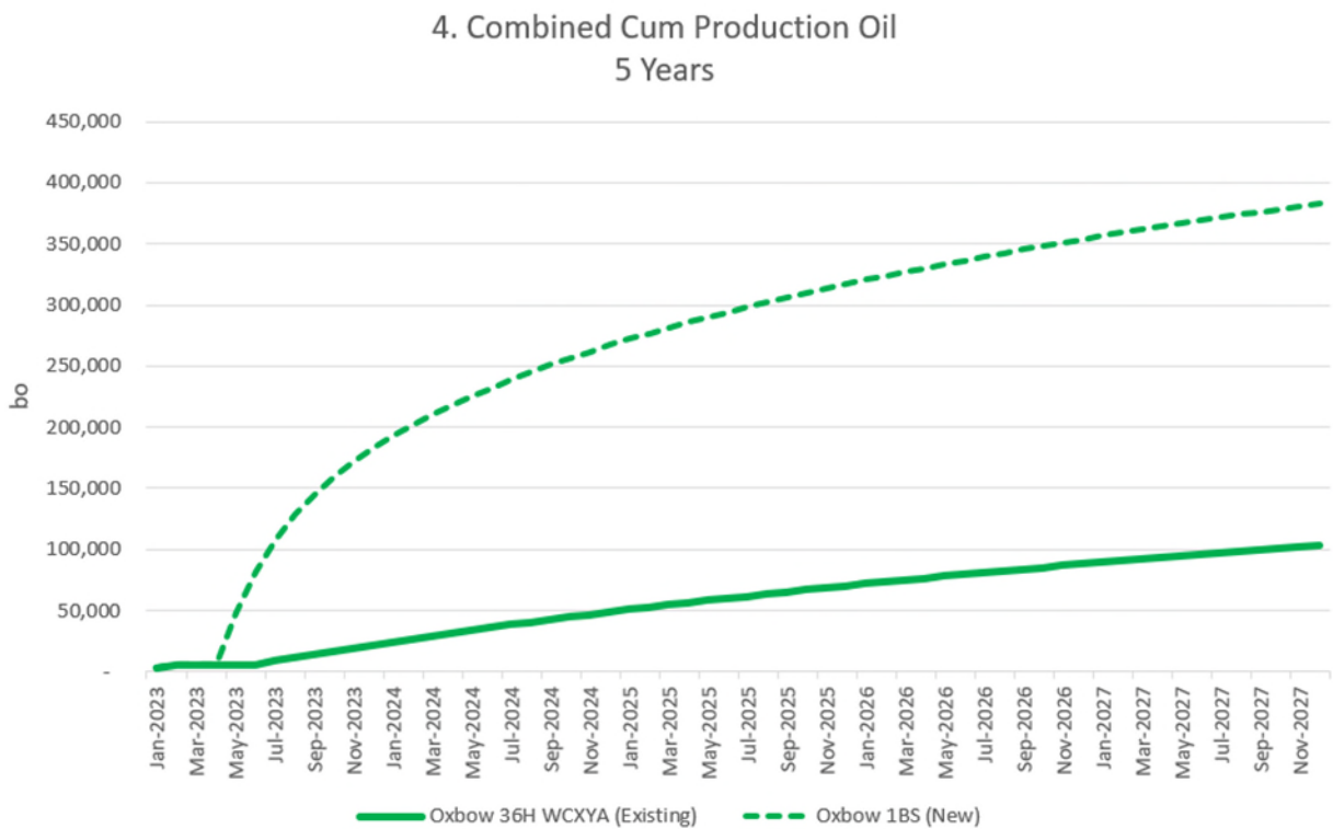
Figure 4- Cumulative oil production by lateral
