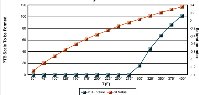
Calcite \text{CaCO}_3
