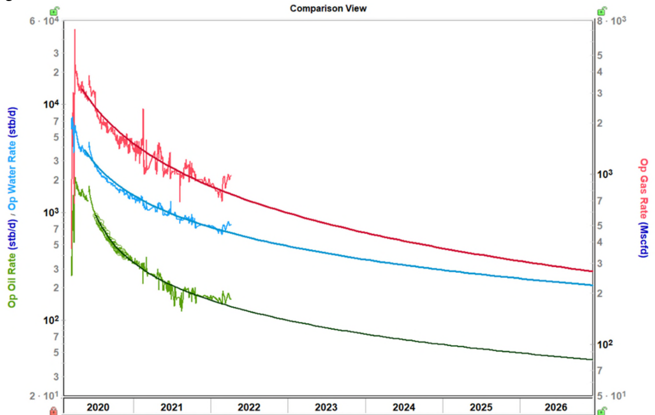
Figure 1- Existing Oxbow 36H Wolfcamp Lateral Production Forecasts
