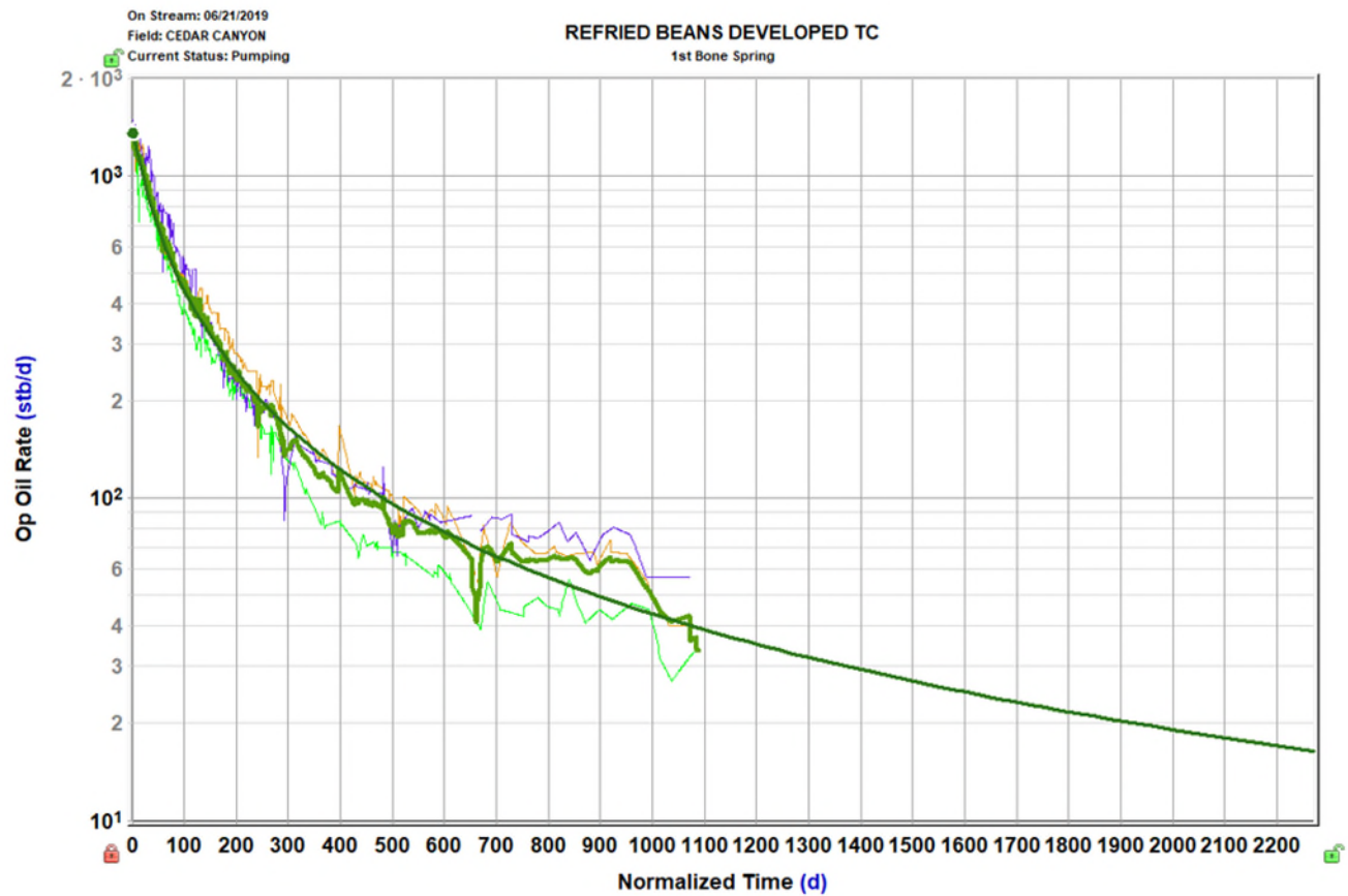
Figure 2- Planned Oxbow 36H Bone Spring Lateral Production Forecast- Oil. Offset production data of 4 wells.
