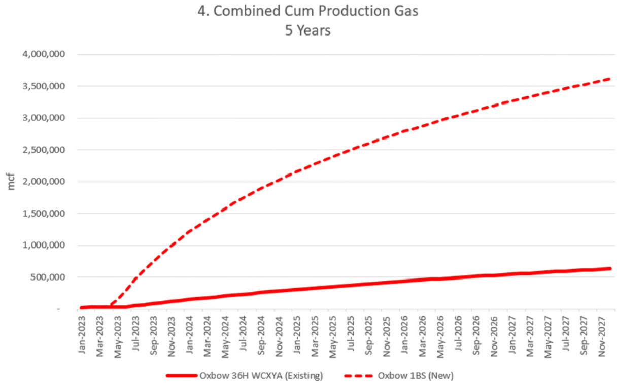
Figure 5- Cumulative gas production by lateral
