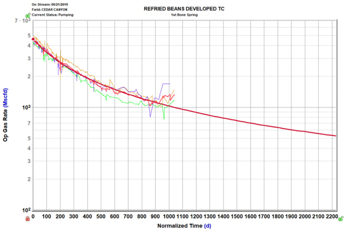
Figure 3- Planned Oxbow 36H Bone Spring Lateral Production Forecast- Gas. Offset production data of 4 wells.
