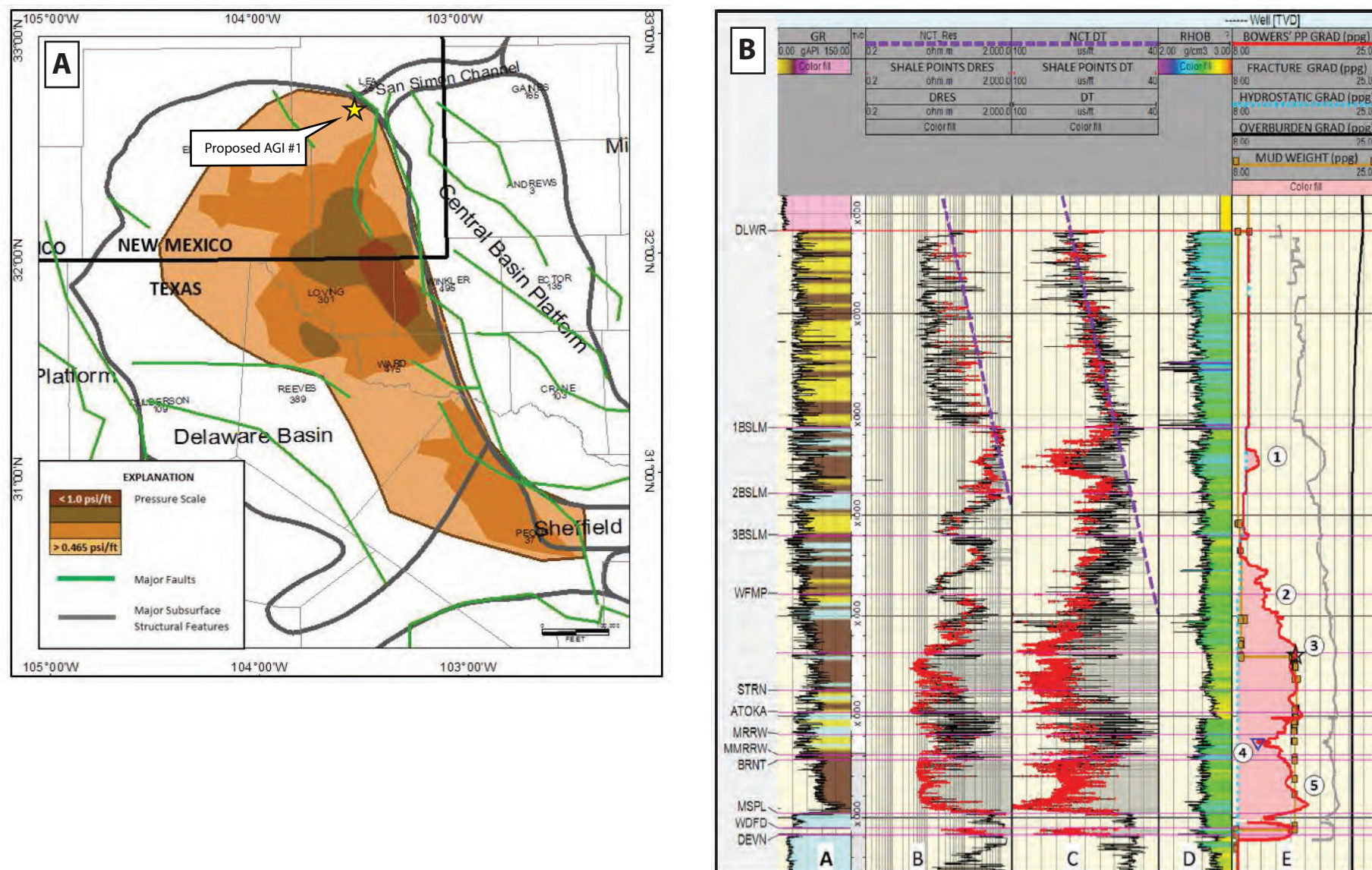
Figure 17. Mapped extent of present day overpressure in the Delaware Basin (Panel A) and example log response (Panel B) illustrating stratigraphic onset of over-pressured intervals and associated drilling fluid densities (modified from Rittenhouse et al., 2016)
