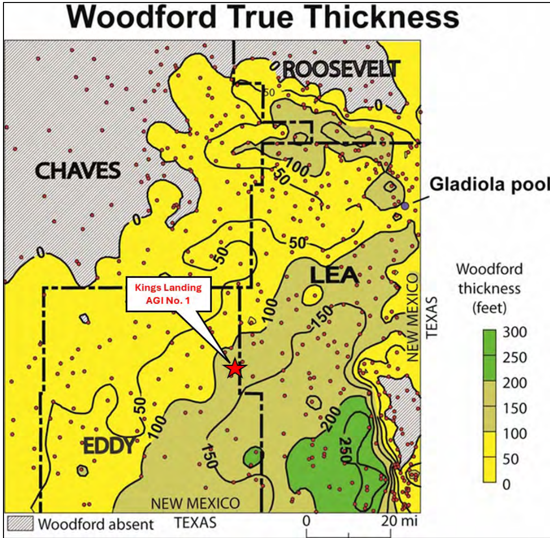
Figure 12 – Regional isopach map of the Woodford Shale in southeastern New Mexico, with the location of the Kings Landing AGI wells represented by the red star (modified from Broadhead, 2011).
