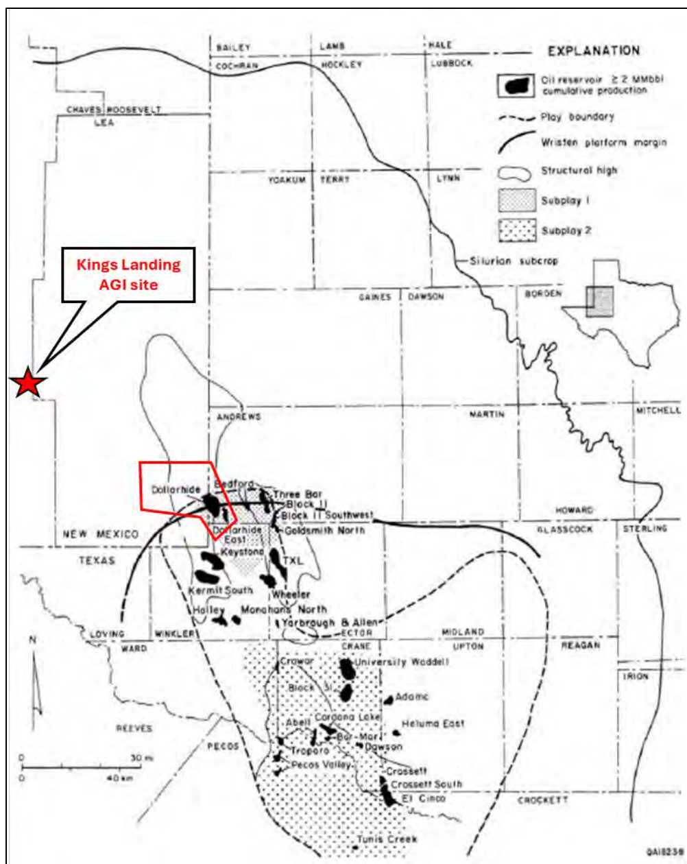
Figure 11 – Location of Dollarhide Field near the Kings Landing AGI site (modified from Ruppel and Holtz, 1994).
