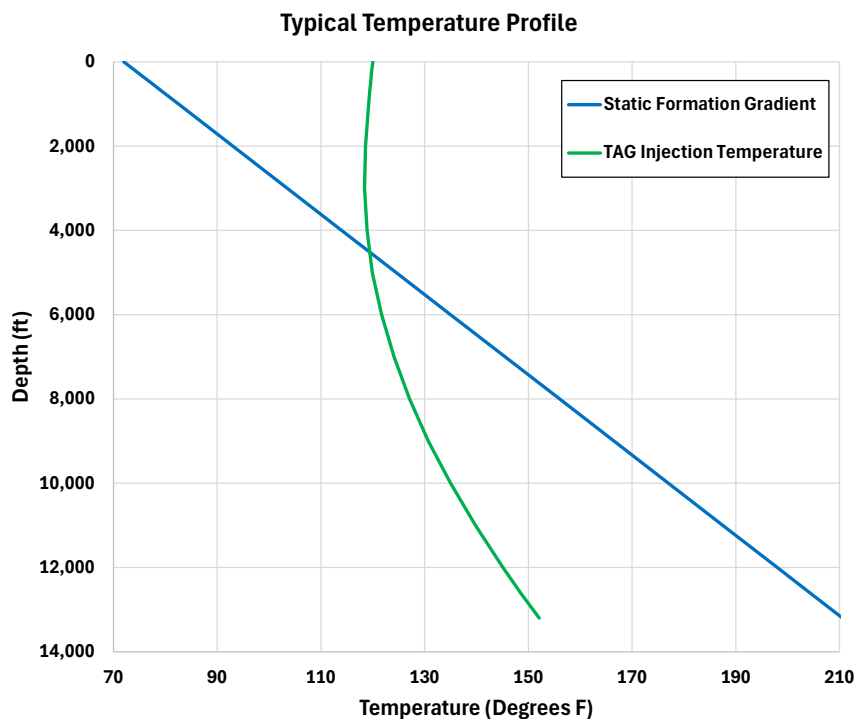
Figure 21 – Temperature Profile
