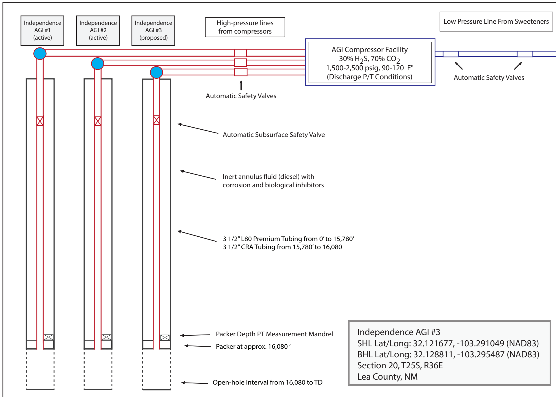
Figure 3. Schematic of surface facilities, proposed Independence AGI #3 and existing Independence AGI # 1 & #2 wells.
