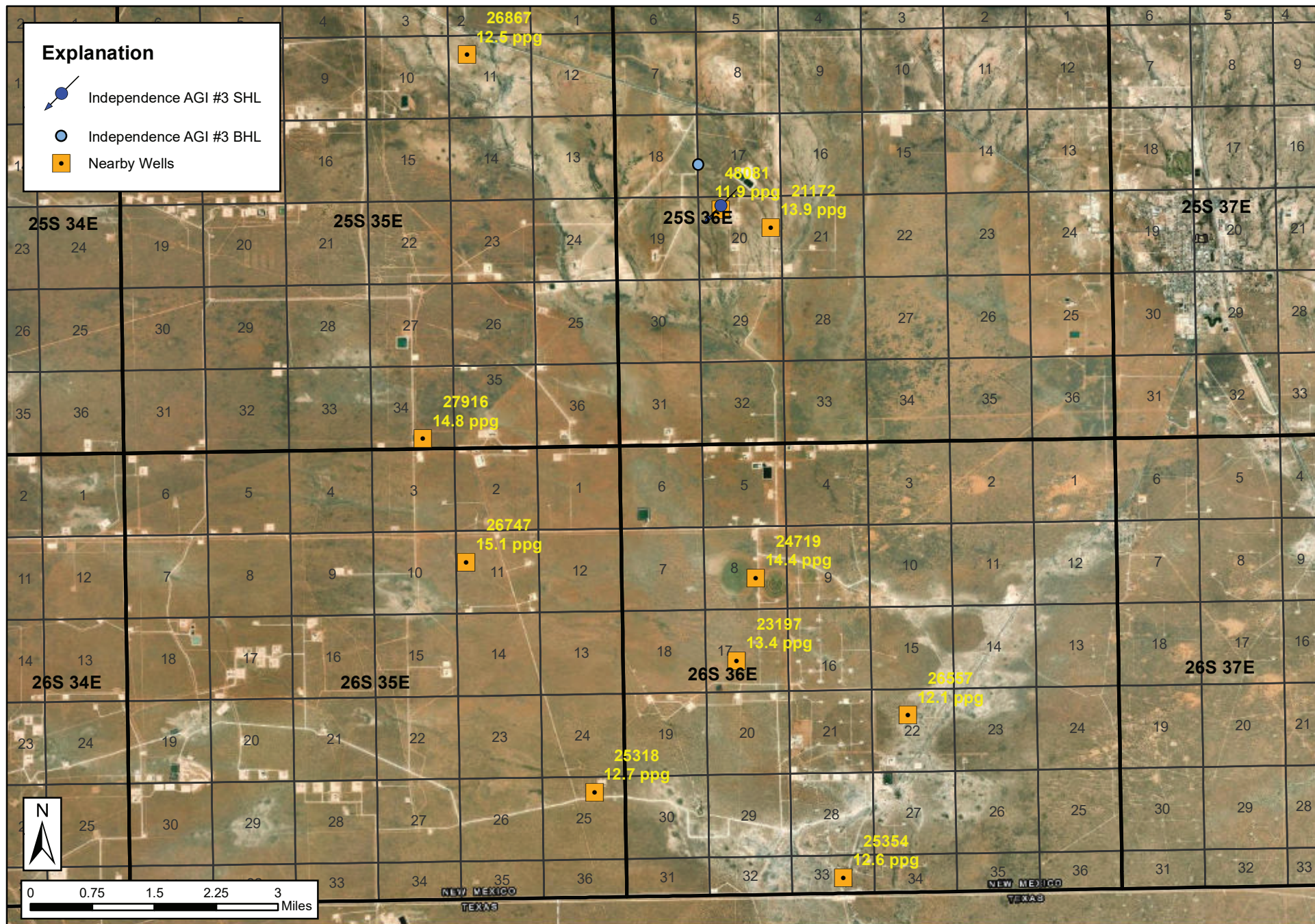
Figure 17. Location map summarizing drilling fluid weights utilized while drilling through overlying productive intervals and strata directly above the proposed injection zone. Labels are the last five digits of the API # (30-025-XXXXX).
