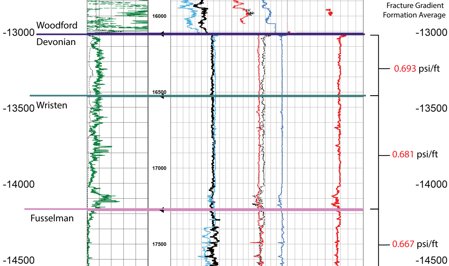
Figure 10. Fracture pressure gradient empirically derived for Independence AGI #1 (red trace). Average fracture gradient estimates range from 0.667 to 0.693 psi/ft. for Devonian through Fusselman geologic strata.
