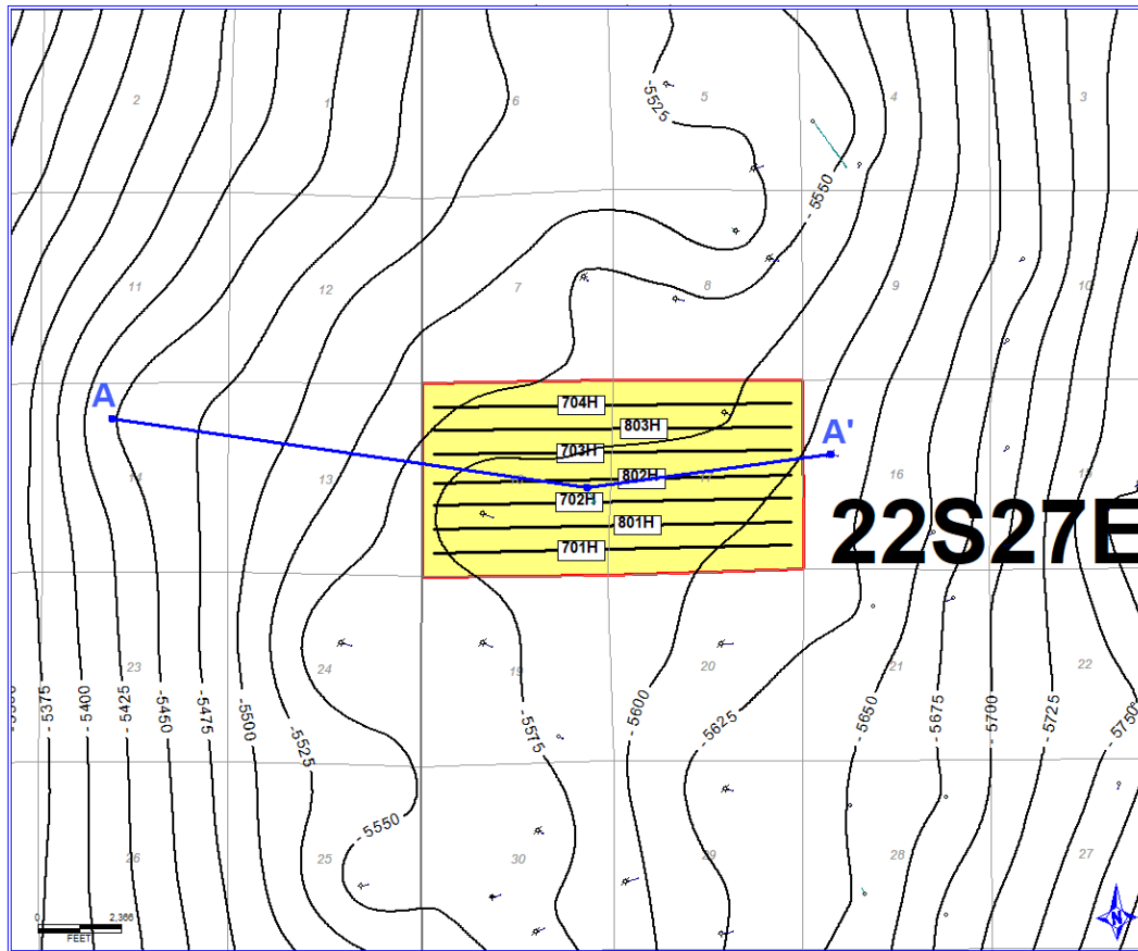
Exhibit B-1 is a structure map showing the depth (subsea) to the top of the Wolfcamp formation, and the location of the proposed wells. The location of the west to east A-A' Cross-Section is also noted.
