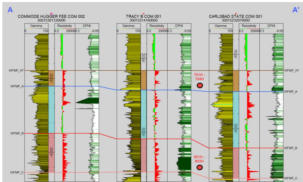
Exhibit B-2 Cross-section A-A'. Stratigraphic cross-section hung on top of Wolfcamp. Target interval indicated by well numbers.
