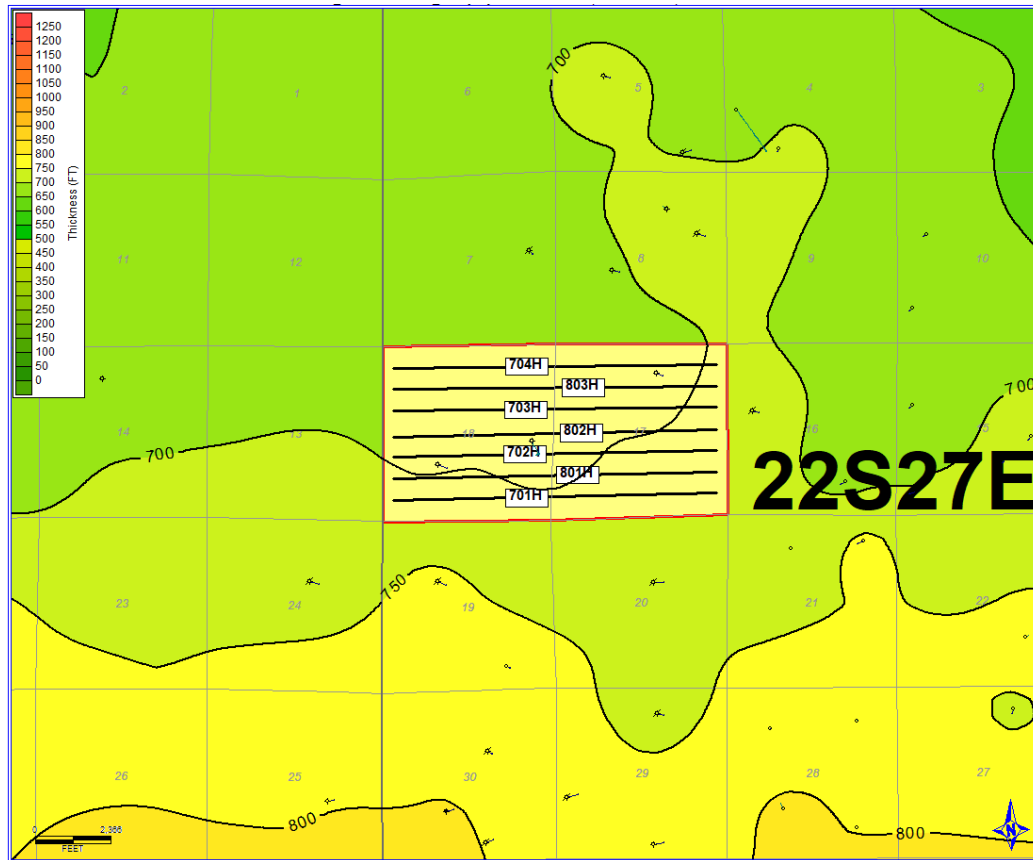
Exhibit B-3 is a gross isochore from the top of Wolfcamp to Wolfcamp C with a 50' contour interval. Map demonstrates continuity and consistent thickness of the target zone.
