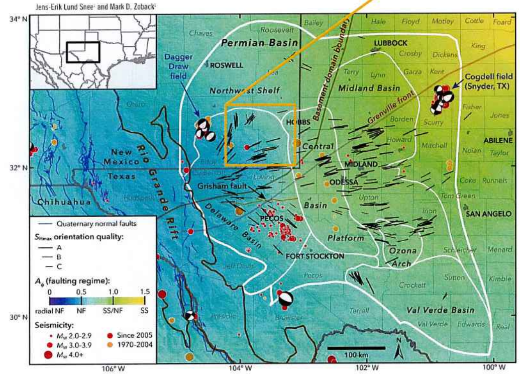
State of stress in the Permian Basin, Texas and New Mexico: Implications for induced seismicity Jens-Erik Lund Snee 1 and Mark D. Zoback 2
