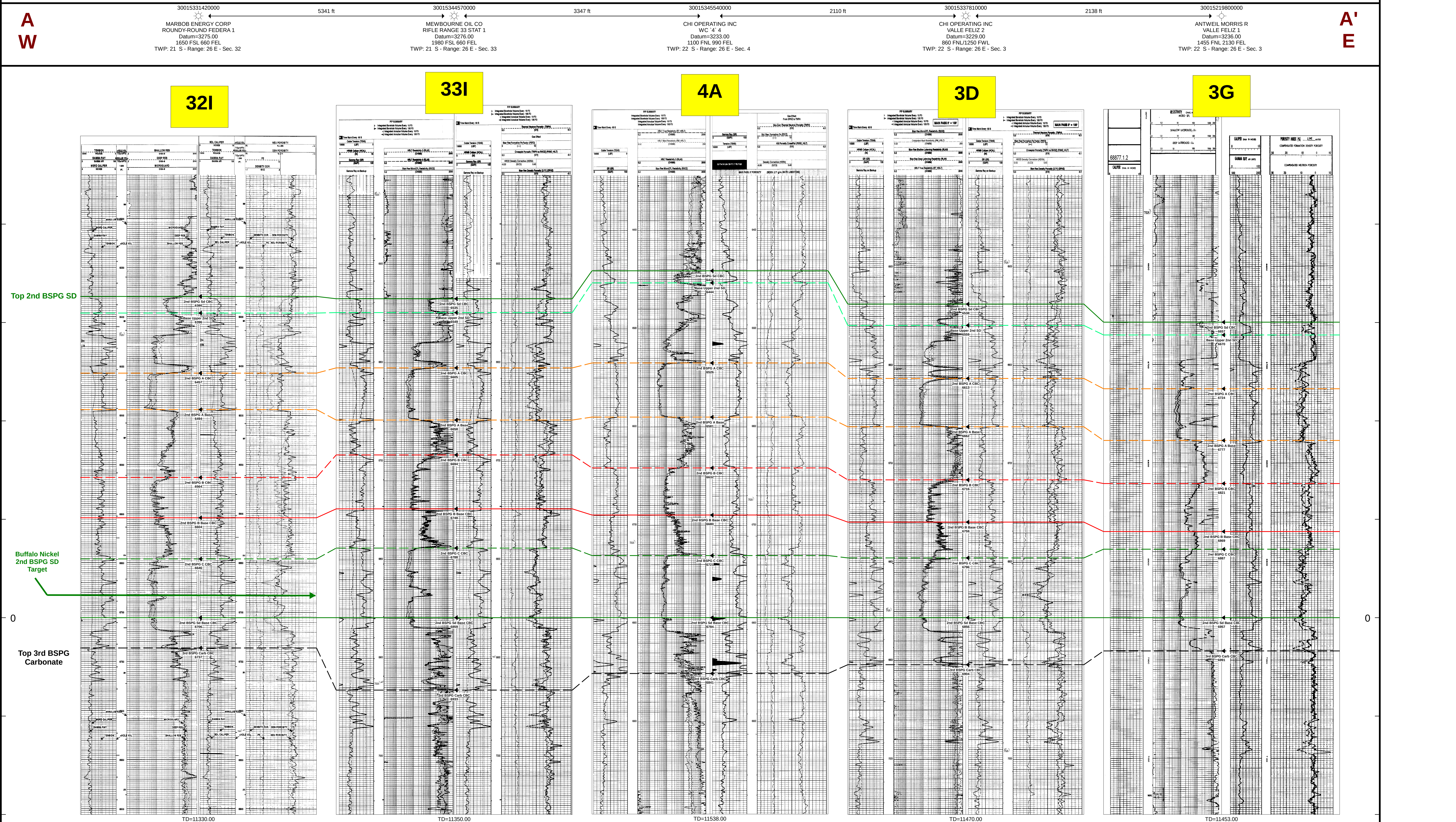
Buffalo Nickel 33/35 State Com 527H 2nd BSPG SD Xsec Exhibit (A-A')
