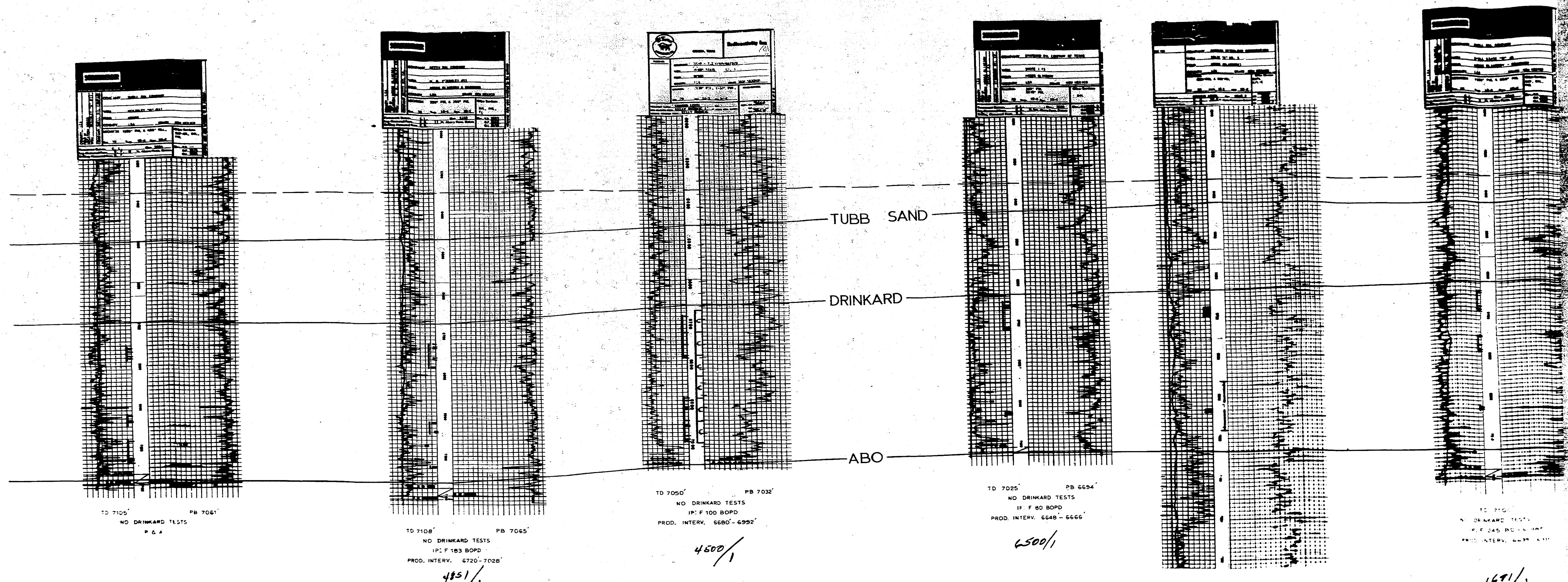
HOBBS DRINKARD POOL STRUCTURAL CROSS SECTION A - A' T18 & 19S R 38E LEA COUNTY, NEW MEXICO Vert. 1 in.=100 ft. Horiz. 1 in.= 400 ft. April, 1972
