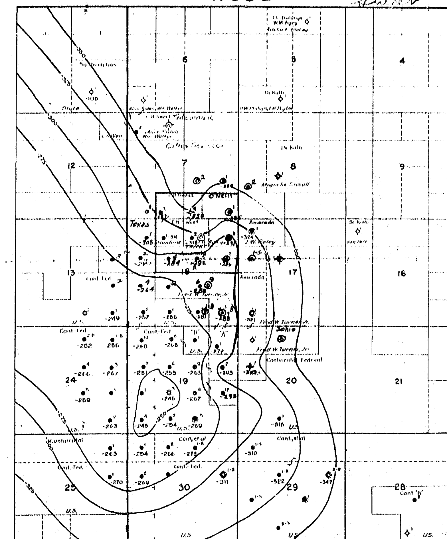
CONTOURS on TOP of "3800' MARKER" SKAGGS-GRAYBURG POOL Contour Interval: 25'-LEA COUNTY, NEW MEXICO — Scale: 2"=1 mile
