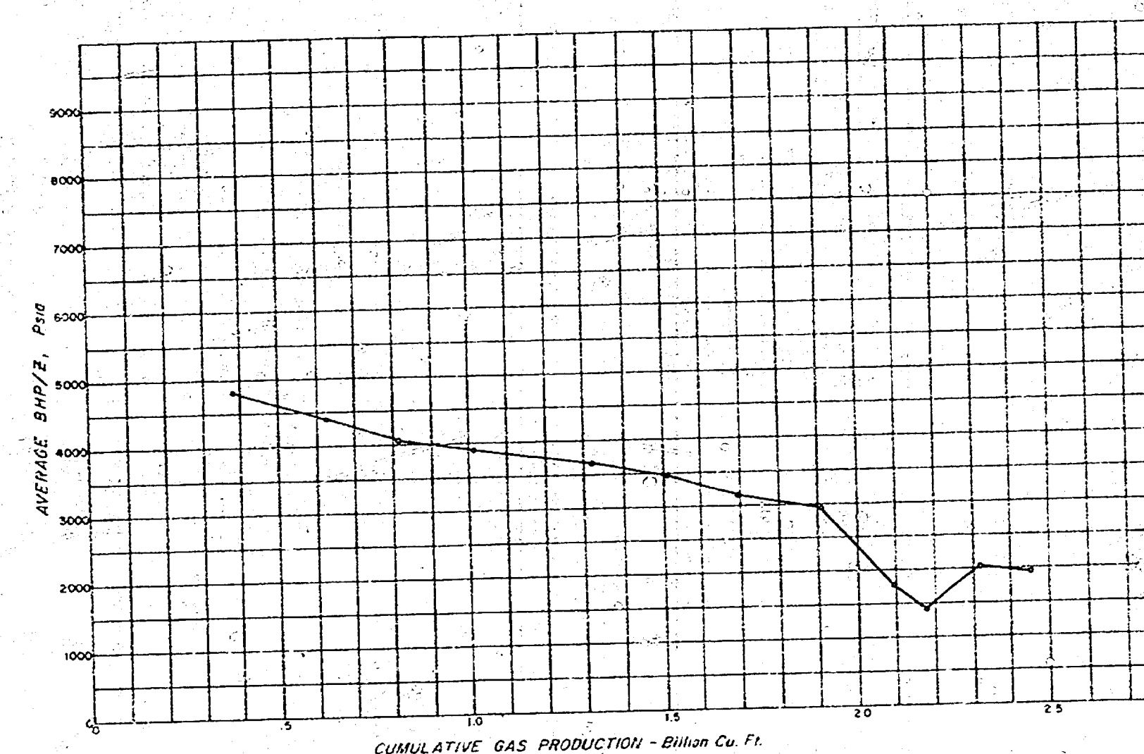
FIGURE NO. PRODUCTION & PRESSURE PERFORMANCE TEXACO NO. 1-CH SL - Little Eddy Unit SO. SALT LAKE POOL LEA COUNTY, NEW MEXICO FELMONT OIL CORPORATION
