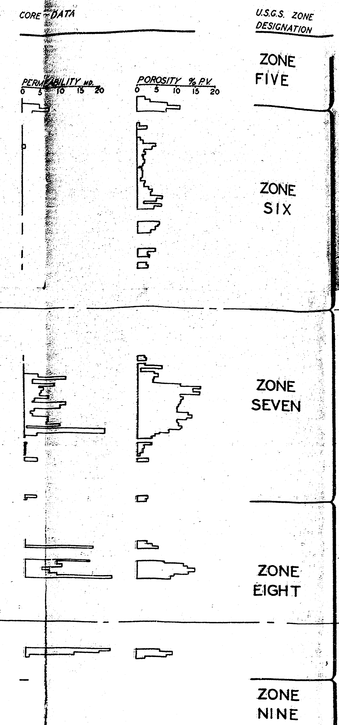
TYPICAL WELL LOG OF THE MALJAMAR OIL POOL WITH CORELATED CORE DATA AND SAMPLE LOG.
