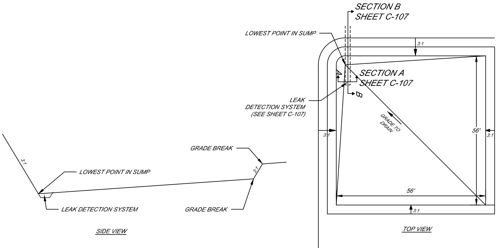
4 C-108 SUMP DETAIL NOT TO SCALE
