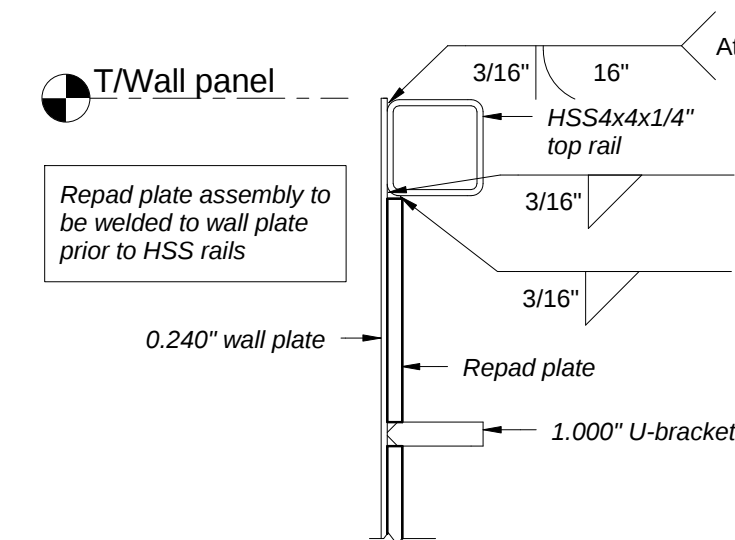
4 Panel Connection Welds - Section SCALE: 1 1/2" = 1'-0"
