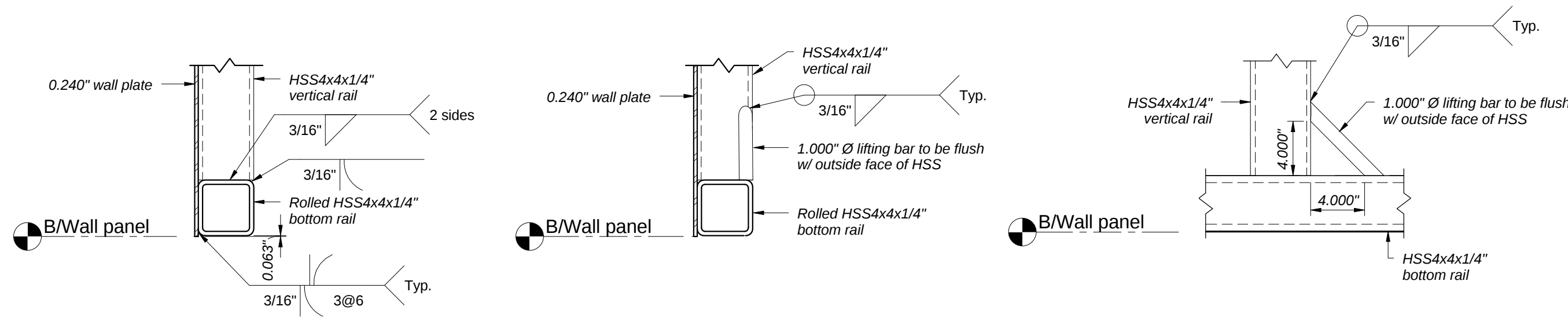
8 Enlarged Detail SCALE: 1 1/2" = 1'-0"
