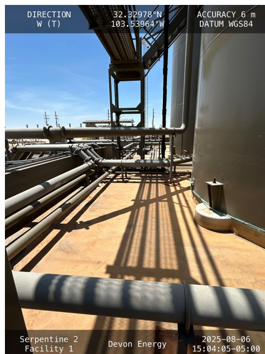
Photo 14 View of southern portion of secondary containment facing west.
