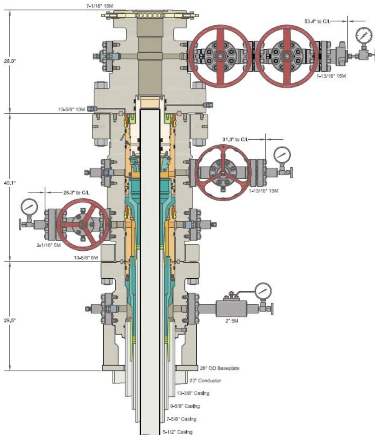
Multi-bowl Wellhead
