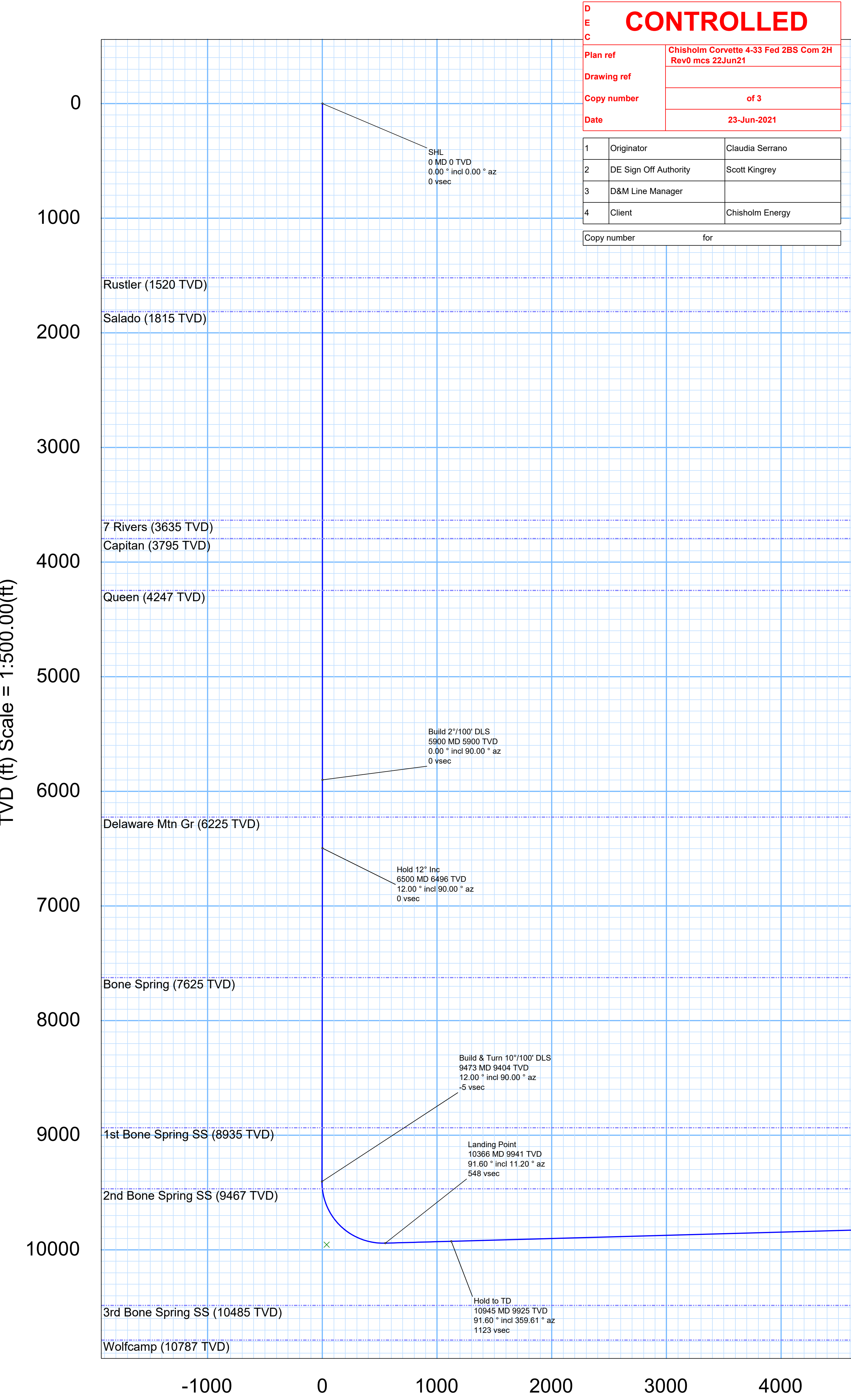
Vertical Section (ft) Azim = 359.61° Scale = 1:500.00(ft) Origin = 0N/-S, 0E/-W
