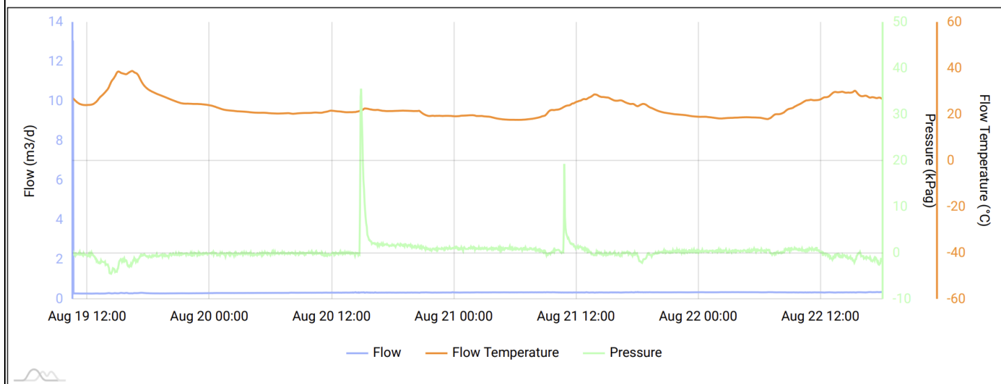
Image 4.1 – Twin Lakes SAU #034L (30-005-60033) Methane Flow/Pressure/Temperature Timeseries
