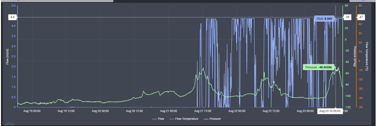
Image 4.1 – Twin Lakes SAU #015 (30-005-62565) Methane Flow/Pressure/Temperature Timeseries & Peak Flow
