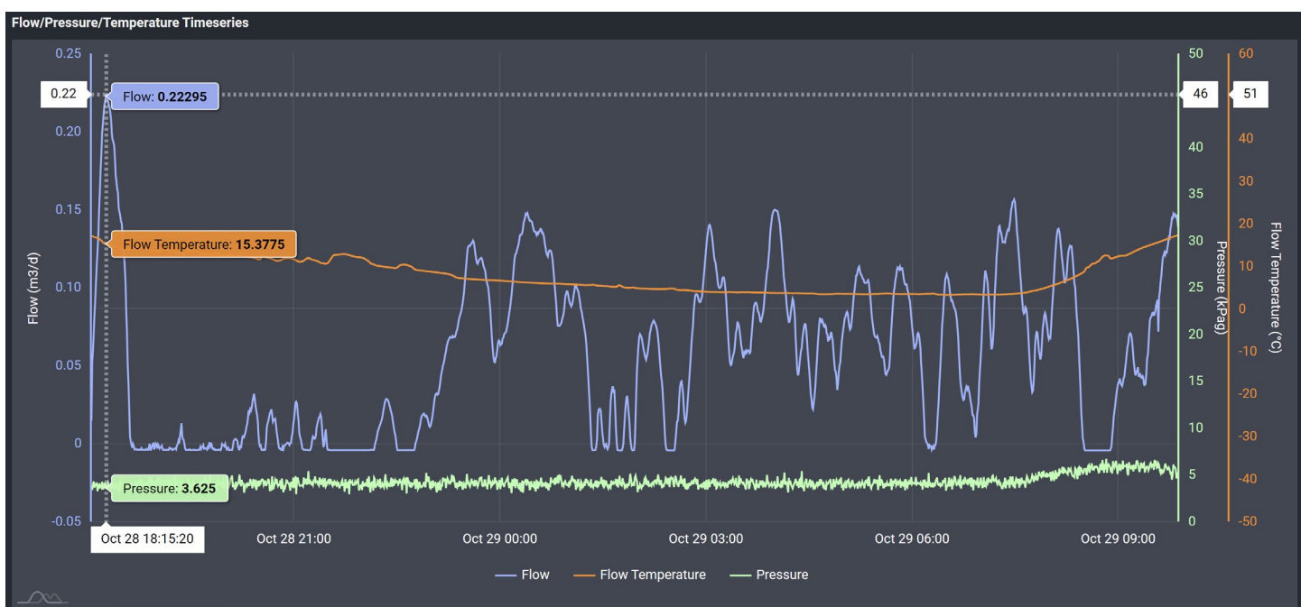
Image 4.2 – Marigold #001 (30-025-32859) Methane Flow/Pressure/Temperature Timeseries &amp; Peak Flow for entire testing period or 15.8-hours.
