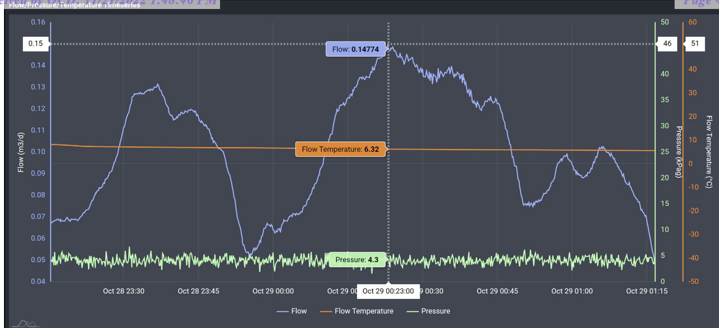
Image 4.1 – Marigold #001 (30-025-32859) Methane Flow/Pressure/Temperature Timeseries &amp; Peak Flow at Interval #1 testing period of 2.0-hours.
