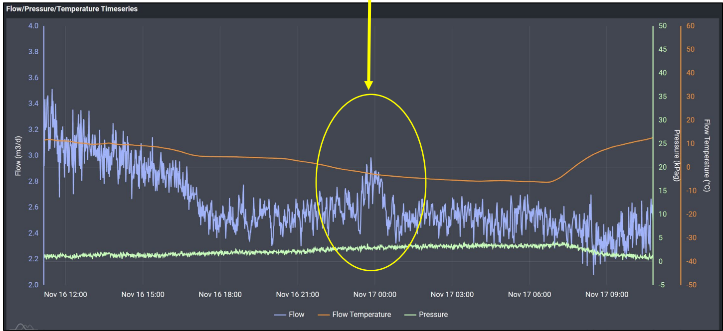
Image 4.2 – Double L Queen #01Y (30-005-60084) Methane Flow/Pressure/Temperature Timeseries & Peak Flow for entire testing period or 23.6-hours.
