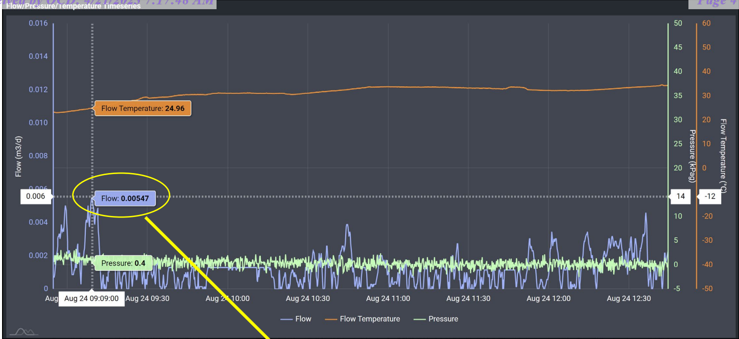
Image 4.1 – TLSA #78K (30-005-60995) Methane Flow/Pressure/Temperature Timeseries & Peak Flow at Interval #1 testing period of 3.8-hours.
