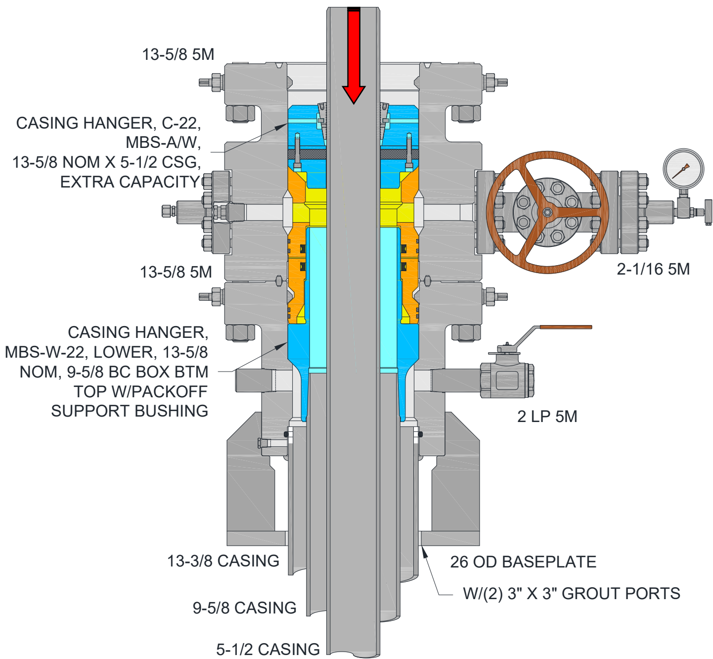
FIGURE 4 – HANGER INSTALLED
