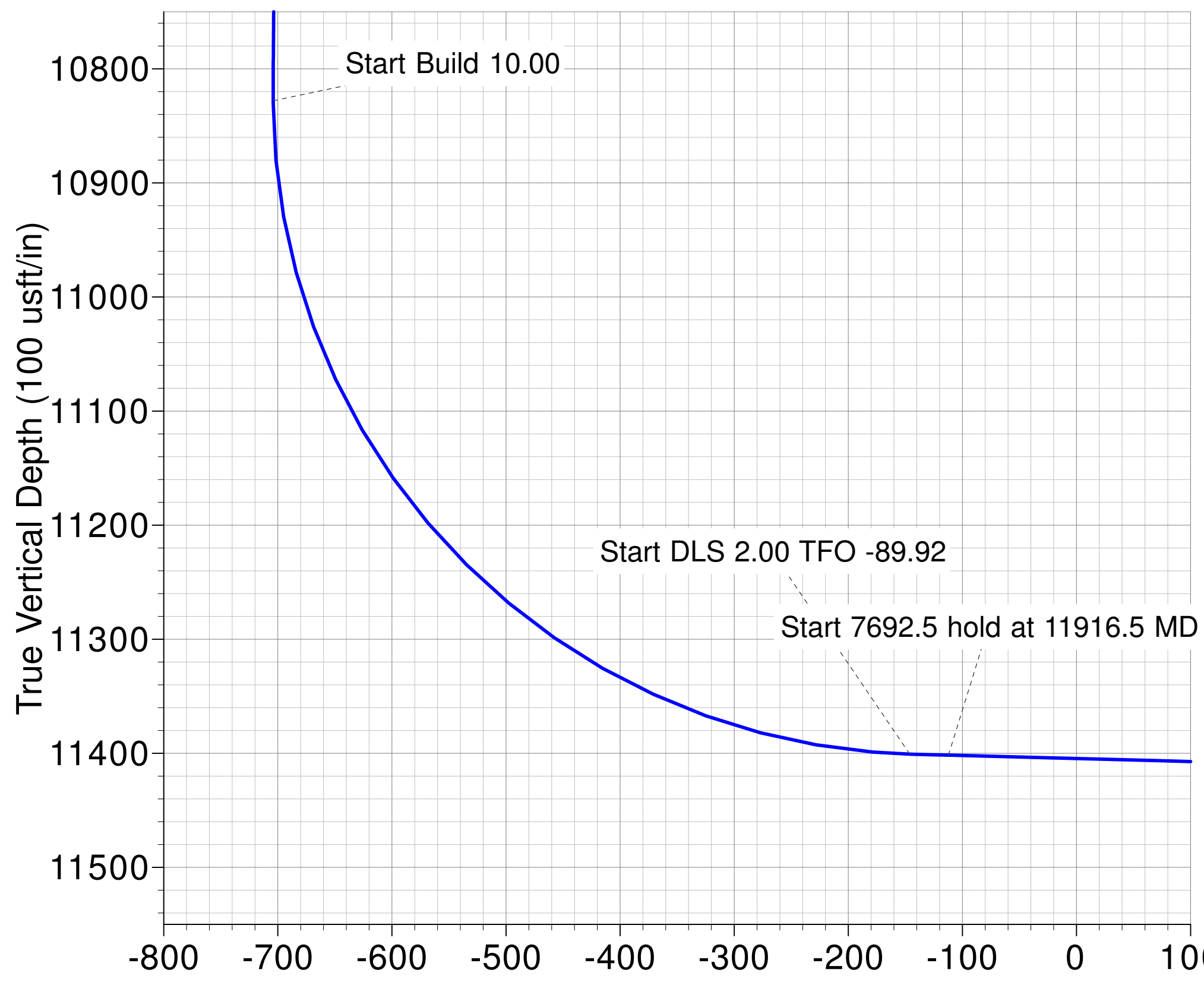
West(-)/East(+) (400 usft/in)
