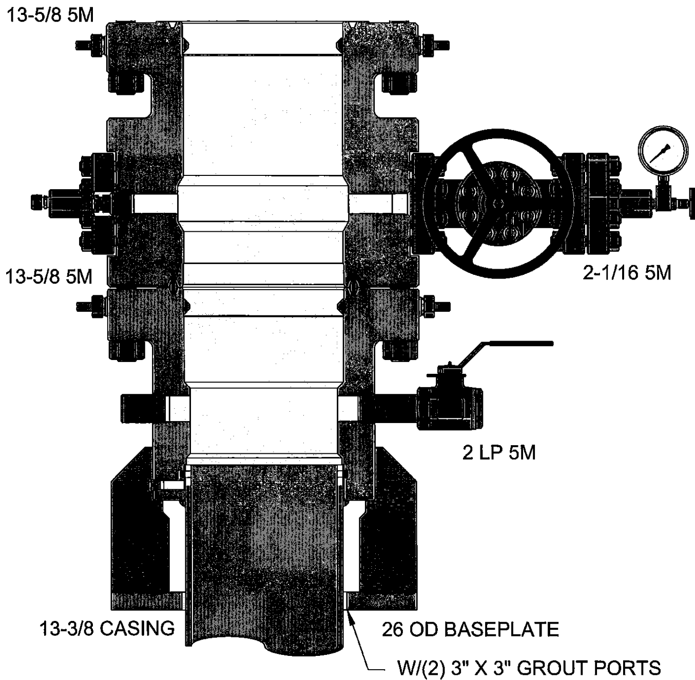
FIGURE 1 – LANDING MULTI-BOWL
