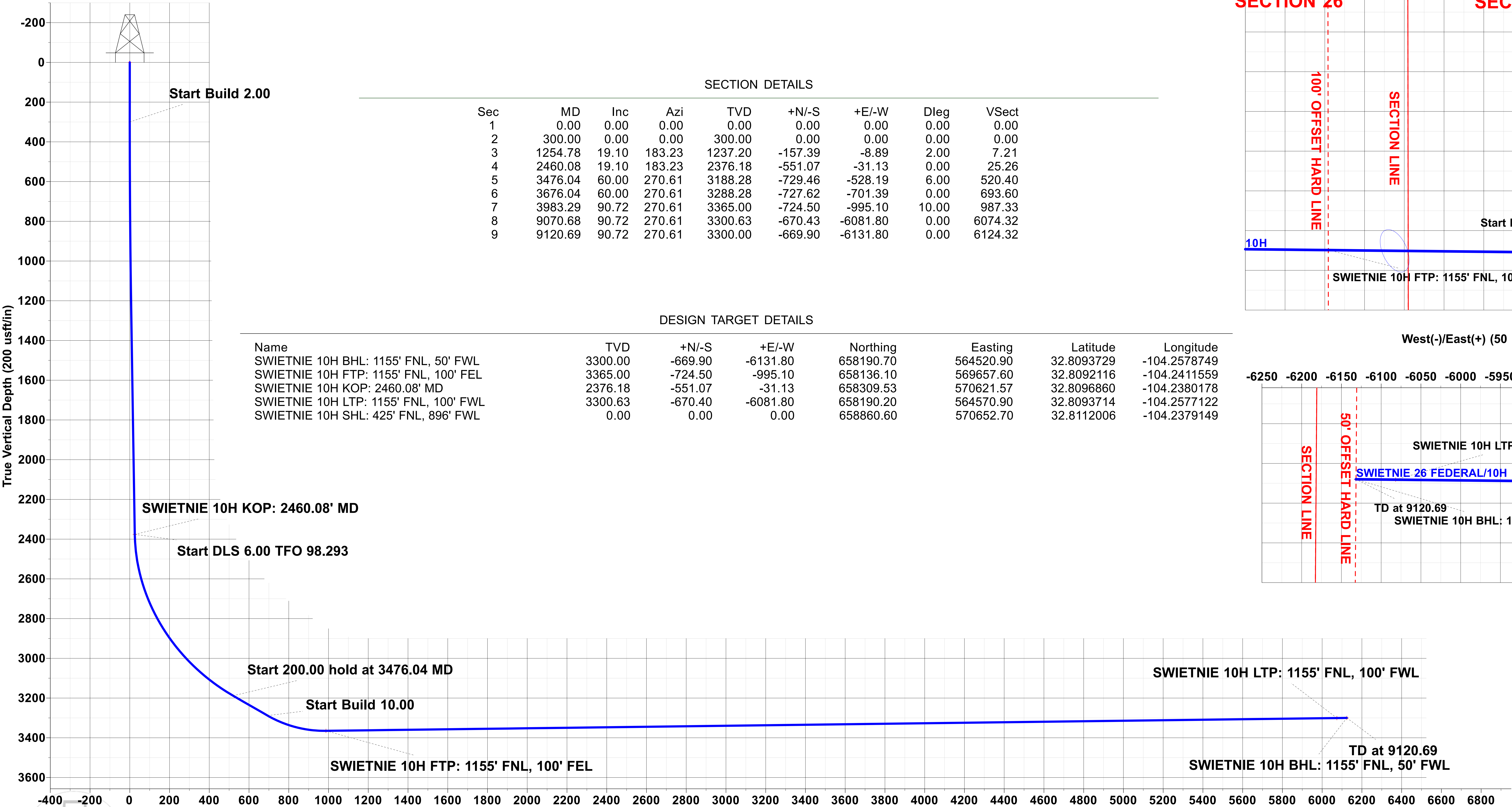
Vertical Section at 270.61° (200 usft/in)
