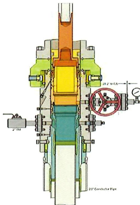
Run 9 5/8" Packoff Test Upper and Lower Seals Engage Lockring Retrieve Running Tool
