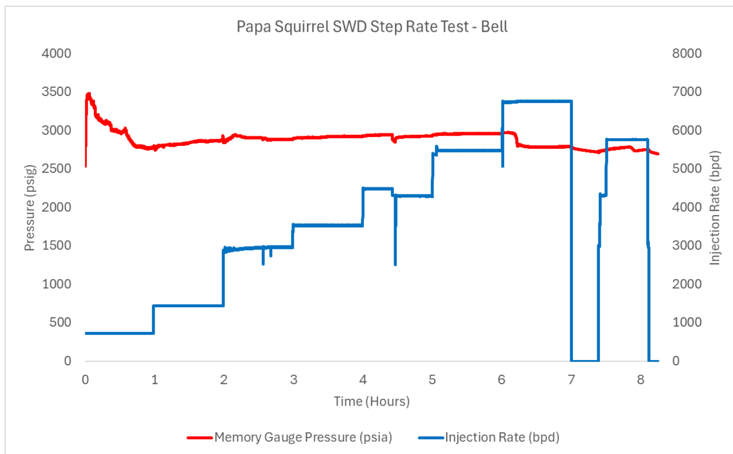
Figure 2 - Injection rate data covering the 1 st 2 steps (0.5 BPM & 1 BPM) was missing on the vendor report plot due to meter communication issues – The actual injection rates during this period is included in the plot above and can be shown from an additional job log
