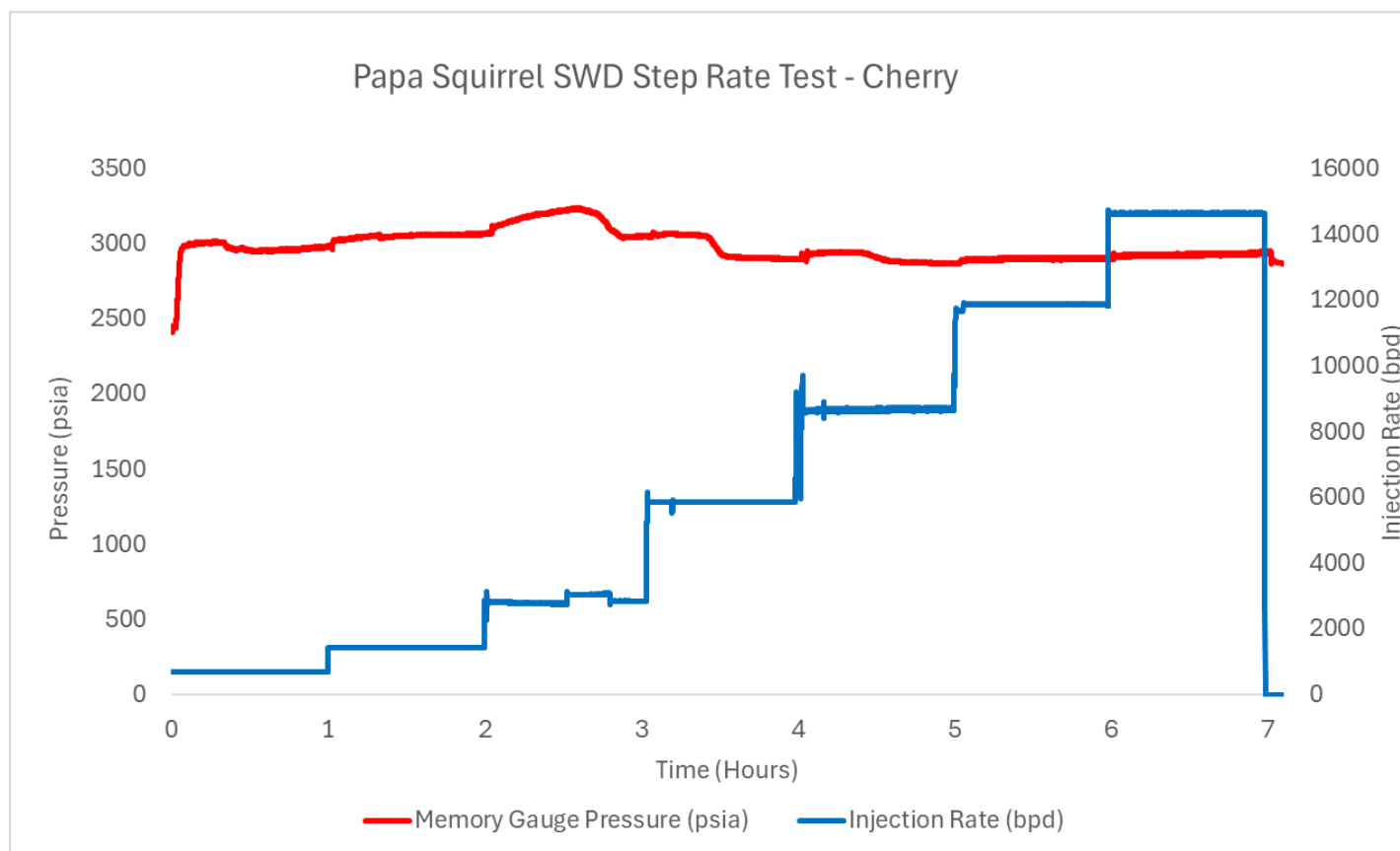
Figure 1 - Injection rate data covering the 1 st 2 steps (0.5 BPM & 1 BPM) was missing on the vendor report plot due to meter communication issues – The actual injection rates during this period is included in the plot above and can be shown from an additional job log
