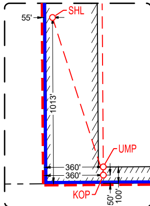
DETAIL VIEW SCALE: 1" = 600'
