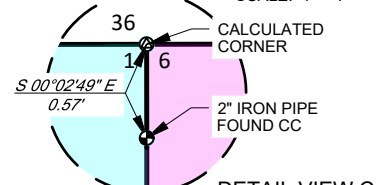
DETAIL VIEW C SCALE: 1" = 1'
