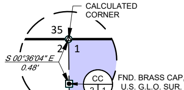
DETAIL VIEW B SCALE: 1" = 1'
