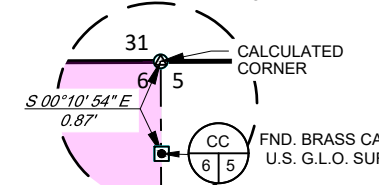
DETAIL VIEW D SCALE: 1" = 1'
