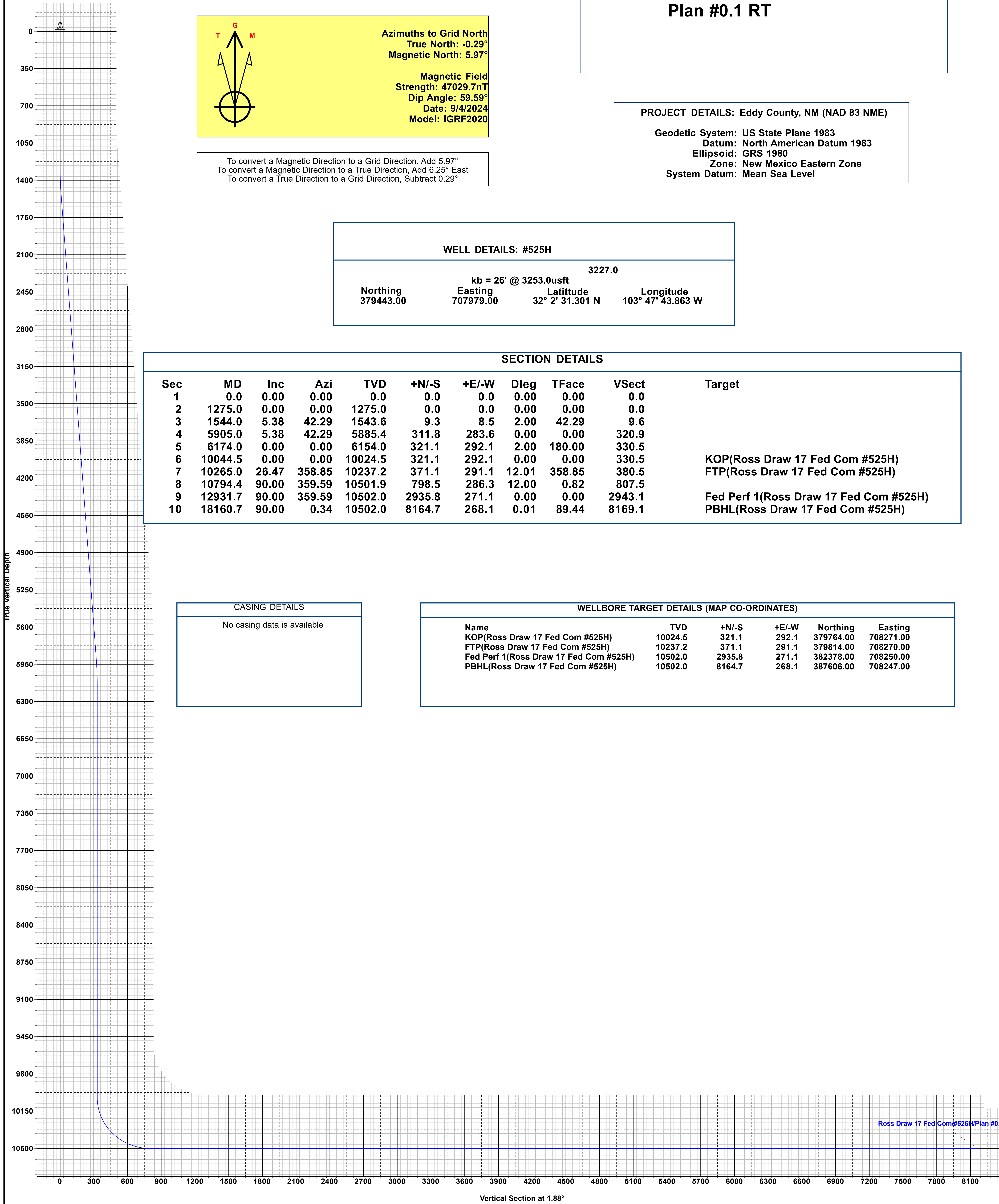
Vertical Section at 1.88°
