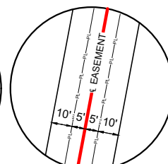
TYPICAL N.T.S. RIGHT-OF-WAY EASEMENT, CONFIGURATION (L6)
