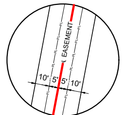
TYPICAL N.T.S. RIGHT-OF-WAY EASEMENT, CONFIGURATION
