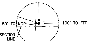
DETAIL "A" (N.T.S.) **MEASUREMENTS FROM MID-SECTION LINE TO KOP(50') AND FTP(100')
